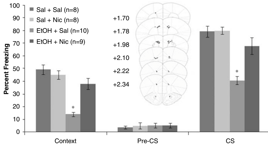
Figure 2 Bilateral nicotine infusion (0.35 \mu\text{g}/0.50\ \mu\text{l} per side) into the anterior cingulate at training and testing ameliorated systemic ethanol-induced (1.0 g/kg) impairments in contextual and cued fear conditioning, but failed to enhance contextual fear conditioning (mean \pm SEM; * indicates significant difference from controls, P < 0.05 ). Center figure represents drug infusion sites.
