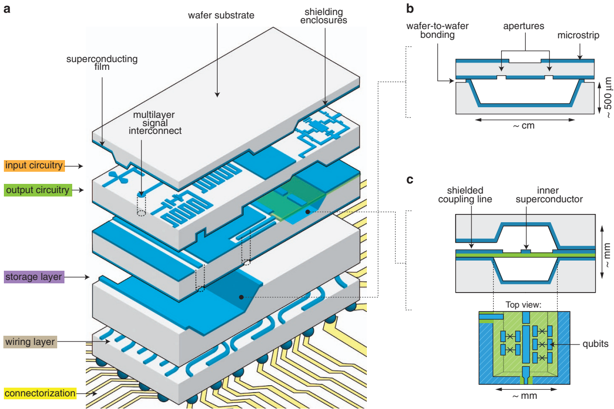
Figure 2. Proposed schematic of a multilayer microwave integrated quantum circuit (MMIQC). (a) Layers are made of silicon wafers with features etched out of the bulk using micromachining techniques to create enclosures that serve as high-Q resonators and as shielding for internal components. Superconducting metallisation (blue) covers the walls of these enclosures and enables low-loss wafer-to-wafer bonding of the layers. Dense planar input/output circuitry, including filters, switches and amplifiers can be embedded in other layers. RF and DC vertical interconnects carry signals between layers, and wire-bonding or ball-grid connection can be used to interface with external control and measurement electronics. (b) A cross-section of the rectangular cavity resonator shows interlayer aperture coupling between the cavity and transmission lines above. (c) 3D superconducting transmission lines could be constructed using membranes (green) in the micromachined structure. Some of these can be populated with qubits and act as a compact low-loss quantum bus.
