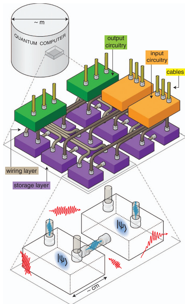
Figure 1. Conceptual sketch of a quantum computer. A large quantum information processor will be composed of many individual modules with precisely managed connections. These modules consist of enclosures approximately a wavelength in size ( \sim cm) containing superconducting circuit elements, including Josephson-junction qubits. Individual quantum states reside in storage modules with minimal loss and high isolation. Modules of input circuitry may include filtered control lines and bias wiring, and output circuitry may include quantum limited amplifiers, filters and switches. Key requirements of the device are addressability via a large number of external connections, indicated by yellow tubes at the surface, and internal selective coupling and isolation, indicated by grey tubes. Unlike the modules, these interconnects can be smaller than a wavelength and require negligible space. Each component is well-isolated from crosstalk and environmental effects (red wave packets) by its enclosure, and components interact only by transmission through shielded channels (blue wave packets). While this sketch shows only a few modules, a quantum processor composed of millions of these components can occupy the payload space of industry standard dilution refrigerators (m 3 ).
