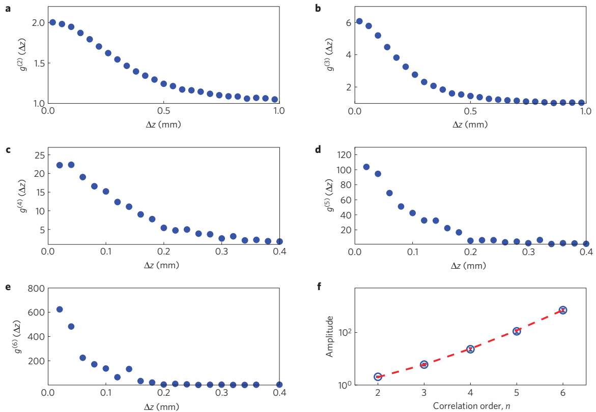
Figure 2 | Many-body correlation functions along the longitudinal direction (temporal dimension on the detector). The data is averaged over the x and y transverse directions using \sim 1 \text{ cm} \times 1 \text{ cm} spatial bins. a–e , A Gaussian fit to the data yields the following peak correlation amplitudes: (a) g^{(2)}(0) = 2.05 \pm 0.09 , (b) g^{(3)}(0) = 6.0 \pm 0.6 , (c) g^{(4)}(0) = 23 \pm 3 , (d) g^{(5)}(0) = 111 \pm 16 , and (e) g^{(6)}(0) = 710 \pm 90 . In f we show the n! scaling (dashed line) of the peak correlation amplitudes.
