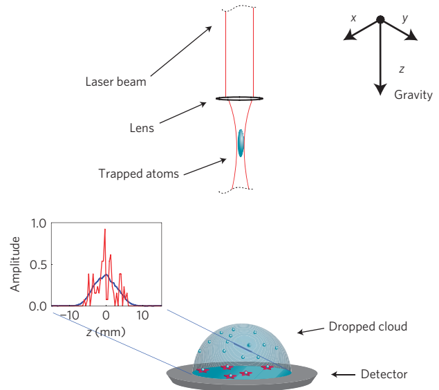
Figure 1 | Schematic of the experiment. An ultracold cloud of atoms is confined in a tightly focused laser beam. When released, the cloud drops \sim 85 cm, where its correlation properties are measured using a single-atom detector. Shown in the inset are the mean (dashed blue line) and a typical single (solid red line) longitudinal profile obtained in the experiment.
