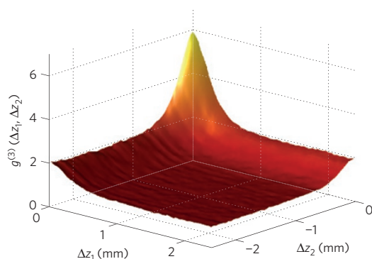
Figure 3 | Surface plot of the three-body correlation function g^{(3)}(\Delta z_1, \Delta z_2) .
