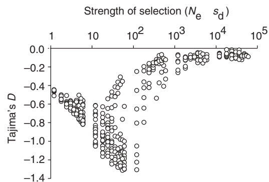
Figure 3 Mean value of Tajima's D under the deleterious mutation model versus the strength of selection ( N_e s_d ). Deleterious mutations of intermediate effect ( N_e s_d = 10 –100) cause the strongest distortion in the frequency spectrum of linked neutral mutations.
