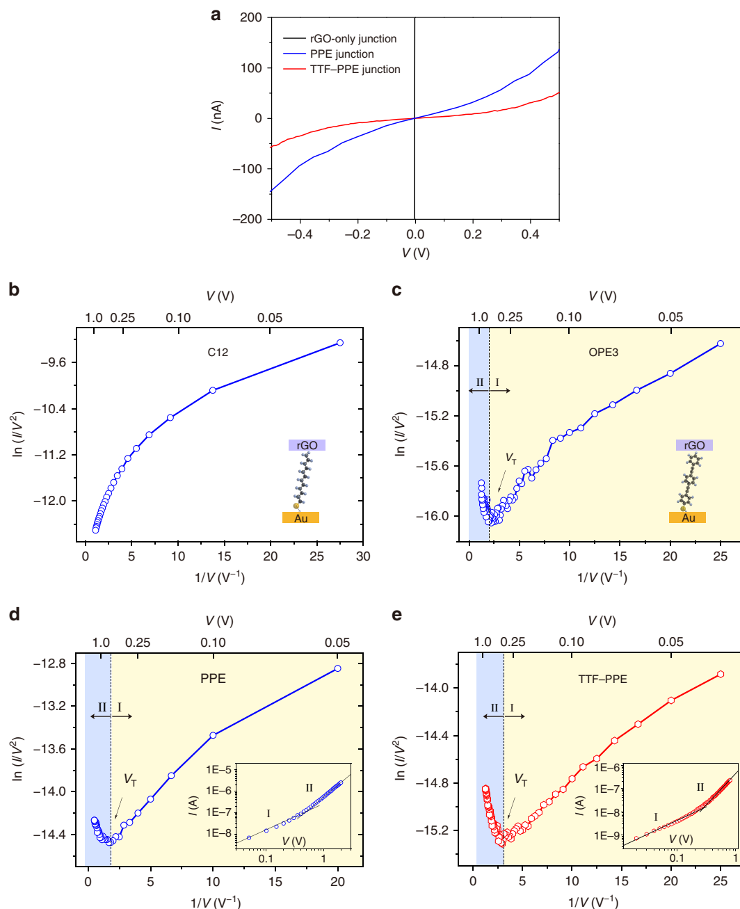
Figure 3 | I - V characteristics of molecular tunnelling junctions. (a) Representative I - V curves of rGO-only junctions and junctions based on PPE and TTF-PPE ultrathin films. (b-e) Fowler-Nordheim plots for I - V traces of junctions based on (b) C12, (c) OPE3, (d) PPE and (e) TTF-PPE. Two distinct regimes (I and II) are clearly observable in c, d and e with a minimum at V_{\text{trans}} . Insets of d and e show log-log plot of representative I - V traces for PPE and TTF-PPE junctions.
