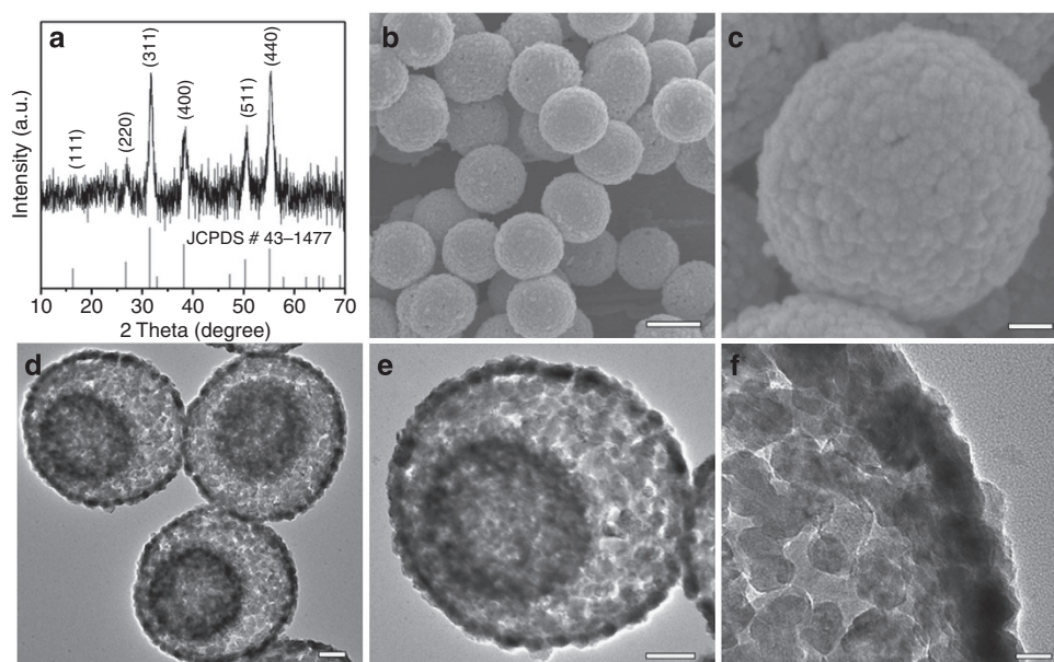
Figure 3 | Materials characterizations of the NiCo 2 S 4 ball-in-ball hollow spheres after annealing in N 2 . (a) XRD pattern, (b,c) FESEM images. Scale bars, 500 and 100 nm, respectively. (d,e) TEM images. Scale bars, 100 nm. (f) Enlarged TEM image of the NiCo 2 S 4 mesoporous shell. Scale bar, 20 nm.
