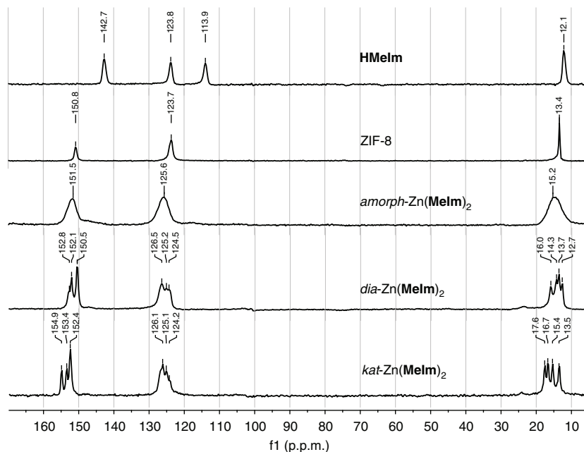
Figure 3 | CP-MAS ^{13}\text{C} SSNMR spectra. CP-MAS ^{13}\text{C} SSNMR spectra for HMelm , ZIF-8, amorph -Zn( MeIm ) 2 , dia -Zn( MeIm ) 2 and kat -Zn( MeIm ) 2 . The weak signal \sim 25 p.p.m. is assigned to the acetic acid additive in the reaction mixture.
