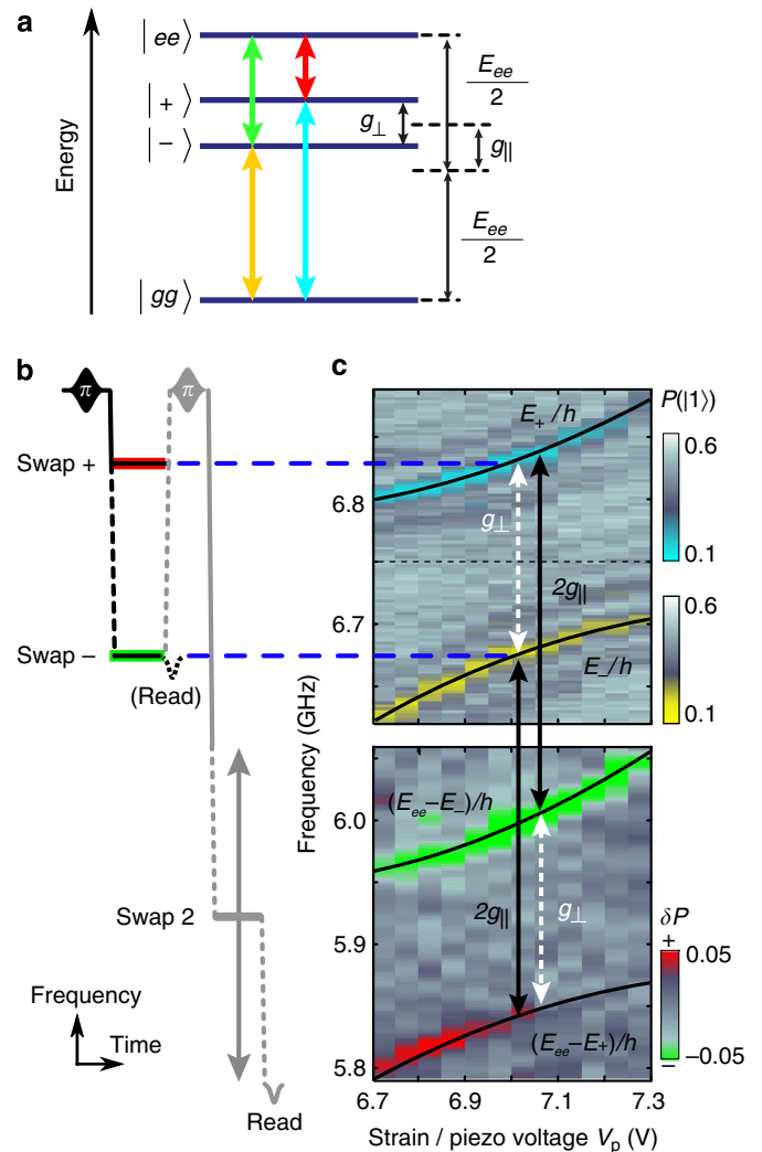
Figure 4 | Exploring the energy level structure for the coupled defect system. (a) Level scheme of the resonantly coupled defect system for an applied strain near the right avoided level crossing of Fig. 3 at V_p \approx 7 V. Energy splitting and offset of the entangled states |\pm\rangle are determined by transversal and longitudinal coupling strengths g_{\perp} and g_{\parallel} , respectively. (b) Pulse sequence used to map out the complete energy level structure. For the upper panel in c , the qubit was measured after the first swap operation at varying frequencies in order to calibrate the entangled states energies. The lower panel was obtained using the complete sequence: preparation of one of the entangled states |\pm\rangle in a first swap, followed by a second qubit excitation and variation of the second swap frequency to reveal the transitions between the entangled states to the fully excited state |ee\rangle . The colour maps were chosen according to the coloured arrows that indicate the corresponding transitions in a . Lines in c are calculated from theory.
