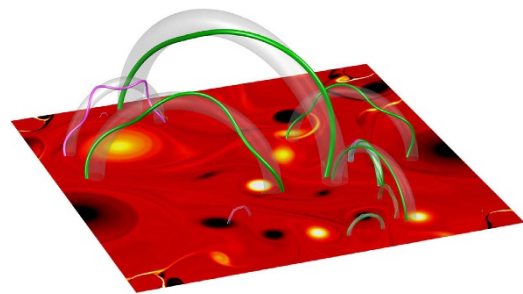
Figure 1 | Configuration of magnetic tubes in the solar corona. The photospheric plasma is in a turbulent state, where yellow (black) areas denote high (low) vorticity regions. The green and pink lines represent the magnetic lines enclosed in the magnetic flux tubes (semi-transparent grey tori). The pink magnetic lines indicate a magnetic flux tube that has reached the critical twist and, therefore, is at the onset of reconnection, about to release its energy as a flare.
