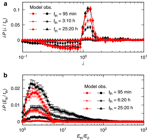
Figure 7 | Flare energies and occurrence times are correlated. (a) The conditional probability difference \delta P(\lambda | t_{th}) = \delta P(E_{i+1}/E_i > \lambda | \Delta t_i < t_{th}) is plotted as function of the parameter \lambda for different t_{th} . Black and red colours represent the observational and numerical catalogues, respectively. Error bars report the s.d. of the probability evaluated for the reshuffled catalogue (see Methods). \delta P is different from zero beyond error bars for a range of \lambda > 1 indicating that, both in the observational and numerical catalogue, for consecutive flares occurring within 3 h the energy of the second flare is larger than the energy of the previous flare. (b) The conditional probability difference \delta P(E_{th} | t_{th}) = \delta P(E_{i+1} > E_{th} | \Delta t_i < t_{th}) as function of the energy threshold E_{th} for different t_{th} . To compare the different catalogues, energies are normalized by E_0 = 1.5 \times 10^{-6} \text{ W m}^{-2} for observational data and E_0 = 150 for numerical data. \delta P is different from zero beyond error bars for energy thresholds E_{th} up to about 10E_0 indicating that, both in the observational and numerical catalogue, as consecutive flares become more distant in time, the probability to find the following flare with energy higher than E_{th} becomes smaller. To convert the numerical units of time, \Delta t_{num} , into physical units, \Delta t , we have used the expression \Delta t_{num} = \Lambda \Delta t / \Lambda_n , where \Lambda_n and \Lambda are the inverse of the average waiting times for the numerical and observational catalogues, respectively.
