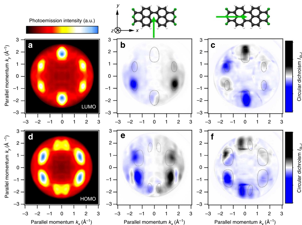
Figure 2 | CDAD for the PTCCA LUMO and HOMO. (a) k_{\parallel} -dependent photoelectron intensity patterns of the PTCCA monolayer on Ag(110) recorded for the LUMO with a photon energy of h\nu = 27 eV as the sum of left- and right-handed polarized light, that is, equivalent to unpolarized light. (b) difference between the k_{\parallel} -dependent intensity patterns recorded with right- and left-circular polarized light, that is, the circular dichroism I(k_x, k_y)_{R-L} for light incidence along the y direction and (c) for light incidence along the x direction. For both plots, dotted iso-intensity contours of a indicate the momentum positions of the molecular structures. (d-f) analogous data for the PTCCA HOMO. On top, the PTCCA molecule is sketched together with green arrows indicating the direction of the incoming light corresponding to the panels below.
