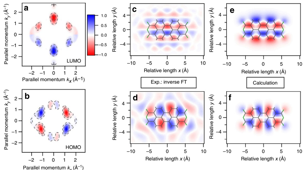
Figure 3 | Reconstruction of the phase distribution and transformation to real space. k_{\parallel} -dependent photoelectron intensity distributions ( h\nu = 55 eV, sum of the left- and right-handed polarized light) of the PTCDA LUMO in a and HOMO in b with superimposed phase (positive: blue, negative: red) derived from the CDAD. The dashed lines indicate iso-intensity contours of the unpolarized signal. The inverse Fourier transformation leads to the sectional real space views of the real part of the LUMO shown in c and the HOMO in d . For illustration, the molecular structure of the PTCDA molecule is superimposed. For comparison, ( e ) and ( f ) show the respective real space orbital pictures derived from ab initio calculations for the isolated molecule.
