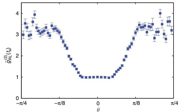
Figure 4 | HOM dip. Normalized atom-atom correlation function \bar{g}_{RL}^{(2)}(t_4) between the two arms of the interferometer, characterizing the HOM effect as a function of the path-distinguishability angle \theta . Error bars denote sampling error from \sim 30,000 stochastic simulations (see Methods). The atom counting bins are rectangular boxes with sides \delta k_x = 0.01k_0 and \delta k_{y,z} = 0.19k_0 , which approximate the widths of the momentum distribution of the initial trapped BEC.
