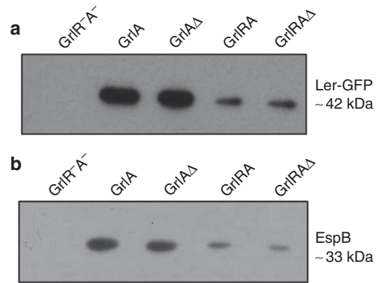
Figure 7 | In vivo functionality of GrIR-GrIA \Delta asymmetric complex. (a) Immunoblot analysis using anti-GFP antibodies to compare the expression of GFP via the ler promoter. The used strains include a deletion mutant of grIRA (control; indicated as GrIR -A- ); this mutant complemented with plasmids expressing GrIA, GrIA \Delta , GrIRA and GIRA \Delta , as indicated above the lanes. All strains contained a compatible GFP-expressing plasmid via the ler promoter. (b) Secreted proteins were concentrated from supernatants of bacterial culture grown in DMEM and resolved using 12% SDS-PAGE. These samples were then transferred to a PVDF membrane and analysed using a monoclonal antibody against representative secretory protein EspB. The strains used are as in a, but all lack the GFP-expressing plasmid. Strains are indicated above the lanes as in a.
