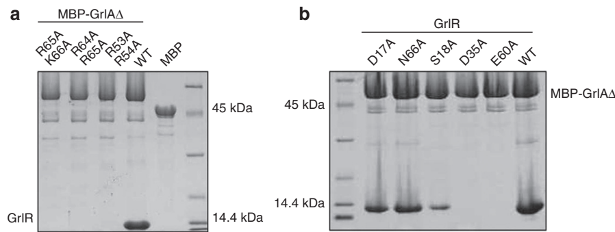
Figure 5 | Role of the key residues in the HTH motif region in GrIR-GrIA \Delta interactions. (a) Pull-down assay to show the binding of GrIA \Delta or mutant variants with GrIR. MBP-GrIA \Delta proteins were bound to amylose beads, incubated with 6His-GrIR overnight and washed. The eluted proteins were separated by 12.5% SDS-PAGE and the gels stained with Coomassie brilliant blue. The GrIA derivatives employed are indicated above the lanes: MBP-GrIA \Delta (R65A K66A), MBP-GrIA \Delta (R64A R65A), MBP-GrIA \Delta (R53A R54A), WT MBP-GrIA \Delta and MBP. (b) Pull-down assay to show the binding of GrIA \Delta with GrIR or the GrIR mutants. The GrIR mutants employed are indicated above the lanes: GrIR D17A, GrIR N66A, GrIR S18A, GrIR D35A GrIR E60A and WT GrIR. The input washes and final elution of the representative mutants are shown in Supplementary Fig. S4a. The additional bands seen on the SDS-PAGE (a) were identified as MBP using peptide mass fingerprint analysis (Supplementary Fig. S4b). Western blot analysis of the pull-down assay (a,b) was carried out using anti-MBP and anti-His antibodies (Supplementary Fig. S5a,d). The pull-down results were confirmed in a co-expression, co-purification pETDuet- grIR-grIA \Delta system and analysed on a 12.5% native gel (Supplementary Figs S6a,b, S7 and S8).
