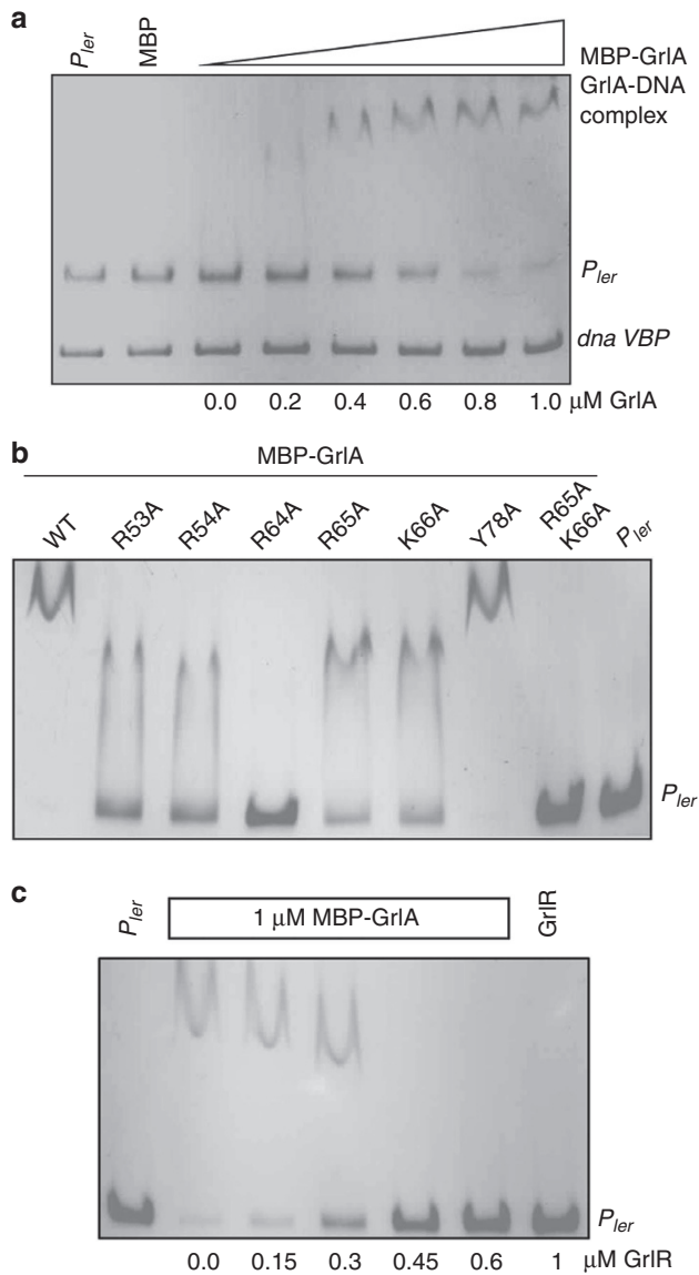
Figure 6 | Interaction of GrIA with the ler regulatory region in vitro . (a) EMSA assay for PCR DNA fragments comprising the ler regulatory region ( ler – 275/ + 217; numbers indicate the number of base pairs upstream and downstream from the functional ATG start codon, respectively) DNA VBP is a non-specific DNA. (b) EMSA assay with substituted MBP-GrIA proteins. PCR DNA fragments comprising the regulatory region ( ler – 275/ + 217) were mixed and incubated with 1.0 \mu\text{M} of purified MBP-GrIA, or with different substituted mutants. Free DNA and protein-DNA complexes were resolved by 5% PAGE and stained with ethidium bromide. The GrIA species used include: WT GrIA, GrIA R53A, GrIA R54A, GrIA R64A, GrIA R65A, GrIA K66A, GrIA Y78A, GrIAR65AK66A and ler pr ( ler – 275/217). (c) Competitive EMSA assay aimed at testing competition between DNA and 6His-GrIR for binding to MBP-GrIA. PCR DNA fragments comprising the regulatory region ( ler – 275/ + 217) were mixed and incubated with 1 \mu\text{M} purified MBP-GrIA for 15 min, then combined with increasing concentrations (0.0, 0.15, 0.3, 0.45 and 0.6 \mu\text{M} ) of 6His-GrIR for an additional 15 min. The complexes and free DNA were separated on a 5% native polyacrylamide gel and stained with ethidium bromide ( ler pr : ler – 275/ + 217).
