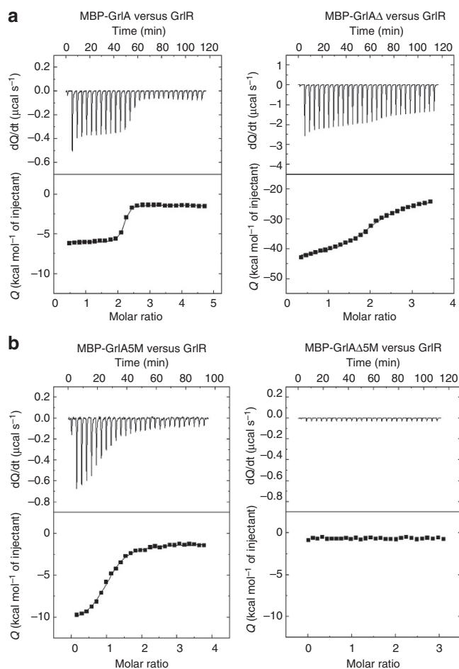
Figure 4 | Role of the C-terminal region and the HTH motif region of GrlA in GrlR–GrlA interactions. (a) The binding affinities of MBP-GrlA/MBP-GrlA \Delta to GrlR were determined using ITC. Representative ITC profiles are shown. The GrlA proteins used are indicated above each panel. The upper part of each panel shows the thermogram (thermal power versus time) after baseline correction and the bottom part of each panel shows the binding isotherm (normalized heat versus molar ratio of reactants) for each injection. The solid lines in the bottom part of each panel show the fit of the data to a function based on a single class of binding site model. (b) The binding affinities of GrlR to MBP-GrlA/MBP-GrlA \Delta with substitutions in the HTH motif region (5M) were determined using ITC (5M refers to substitutions at R53A, R54A, R64A, R65A and K66A). The binding constants ( K_a and K_d ), number of binding sites ( N ), enthalpy ( \Delta H ) and entropy ( \Delta S ) are provided in Supplementary Table S1.
