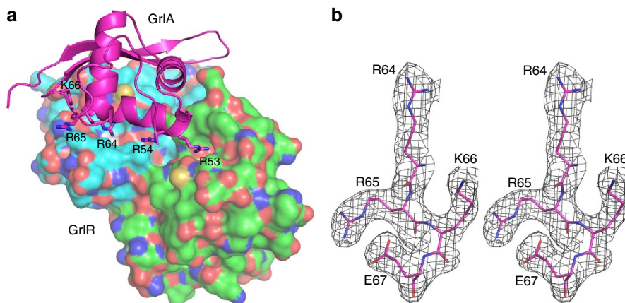
Figure 3 | Structure of the GrlR-GrlA \Delta interacting surface. (a) The GrlR dimer is shown in surface representation and GrlA \Delta is shown as a cartoon. The interacting residues of GrlA \Delta are shown as sticks. (b) Final 2 Fo - Fc electron density map (contoured at 1 \sigma ) for the key residues of GrlA \Delta .
