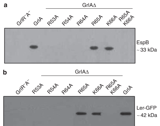
Figure 8 | In vivo analysis of the importance of key HTH motif residues in GrIA-DNA binding. (a) Secreted proteins were concentrated from supernatants of bacterial culture grown in DMEM and resolved in 12% SDS-PAGE. The samples were then transferred to a PVDF membrane and analysed using polyclonal antiserum against representative secretory protein EspB. The used strains include a deletion mutant of grIRA (control) (indicated as GrIR -A- ); this mutant complemented plasmids expressing GrIA or different GrIA \Delta substitutions, as indicated above the lanes (b). Immunoblot analysis using anti-GFP antibodies to compare the expression of GFP via the ler promoter. The used strains are similar to those described in a, with the exception that all contain a compatible GFP expression plasmid via the ler promoter. Strains are indicated above the lanes.
