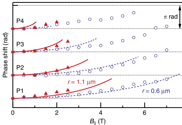
Figure 5 | Radius dependence of the geometrical phase shift with an in-plane field B_{\parallel} . The vertical axis represents the phase shift of the AC oscillations in units of radians (one period of the AC oscillations corresponds to 2\pi rad). Experimental results are plotted as the open (filled) symbols for r = 0.6 \mu\text{m} ( 1.1 \mu\text{m} ) sample. The lines are the perturbation theory, with r = 0.6 \mu\text{m} (dashed) and r = 1.1 \mu\text{m} (solid). The notations P1-P4 represent the peak and dip positions of the AC phase (see Fig. 3).
