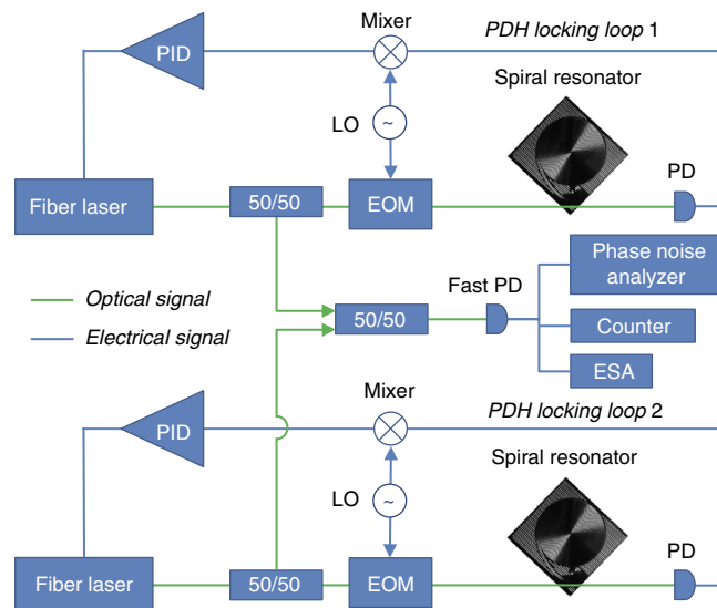
Figure 3 | Experimental setup. Two, fibre lasers independently locked to high-Q spiral reference cavities using Pound-Drever-Hall (PDH) locking systems. Each PDH locking loop includes a photodiode (PD), electro-optic modulator (EOM), local oscillator (LO) and proportional-integral-differential feedback controller (PID). The outputs of the separately locked lasers were combined on a photodetector and the resulting photocurrent was analysed using an electrical spectrum analyser (ESA), a frequency counter and a phase-noise analyser. All components are on the same optical table.
