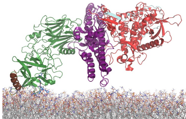
Figure 4 | Model of BoNT binding to the neuronal membrane. The H C (green), with its bound Syt-II (brown) and GD1a (blue), is from this study, while the H N (purple) and LC (red) is superimposed using the structure of the entire BoNT/B (PDB code: 2NPO). The protein orientation is restricted by the binding of the two receptors. The structure presented here supports the entry of the translocation domain into the membrane with the end of the long helixes first 22,28 . The regions linking both the protein receptor and ganglioside receptor to the membrane does allow for a certain degree of flexibility of the toxins orientation.
