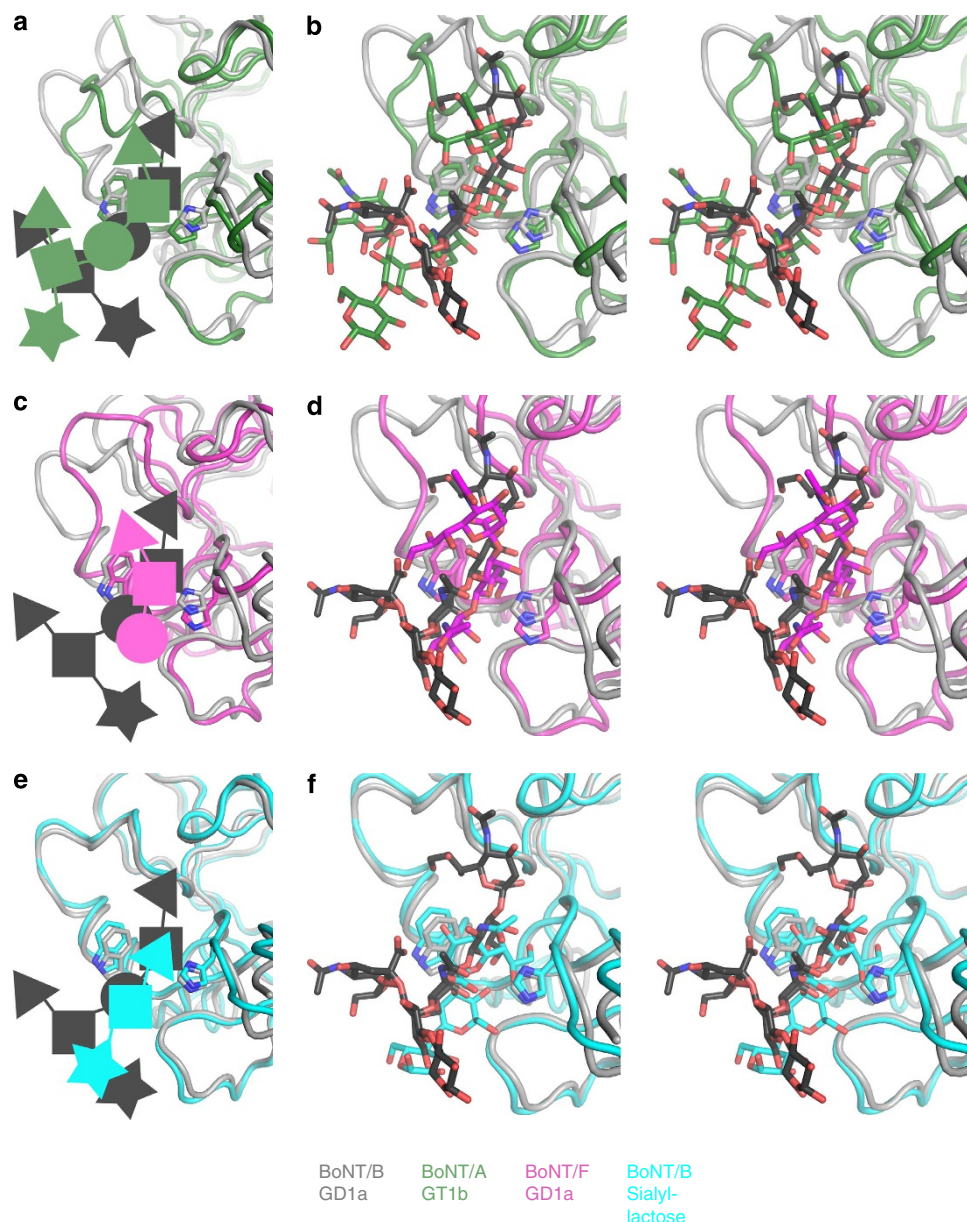
Figure 2 | Comparison of the ganglioside binding to BoNT/B, BoNT/A and BoNT/F. The residues corresponding to W1262 and H1241 are shown in all structures. In the schematic panels (a,c,e) the individual sugar moieties are depicted as follows; triangles, Sia; rectangles, Gal; circle, GalNAc; star, Glc. In all panels, BoNT/B with GD1a bound is depicted in grey and dark grey, respectively. The right-hand panels (b,d,f) are stereo figures of the GBS. (a,b) Comparison to BoNT/A with GT1b (green, PDB code: 2VU9). (c,d) Comparison to BoNT/F and its bound GD1a (magenta, PDB code: 3RSJ). (e,f) Comparison to BoNT/B and its bound sialyllactose (cyan, PDB code: 1F31).
