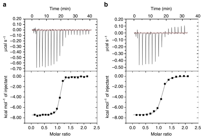
Figure 5 | ITC titrations of Syt-II to BoNT/B. Representative ITC titrations of Syt-II to BoNT/B, without (a) and with (b) pre-incubation of 75 \mu\text{M} GD1a. (a) K_D = 0.14 \pm 0.05 \mu\text{M} , (b) K_D = 0.18 \pm 0.06 \mu\text{M} . The error is the s.d. on at least two independent measurements. The baseline above zero in b is due to a slight buffer mismatch, and does not influence the calculated values.
