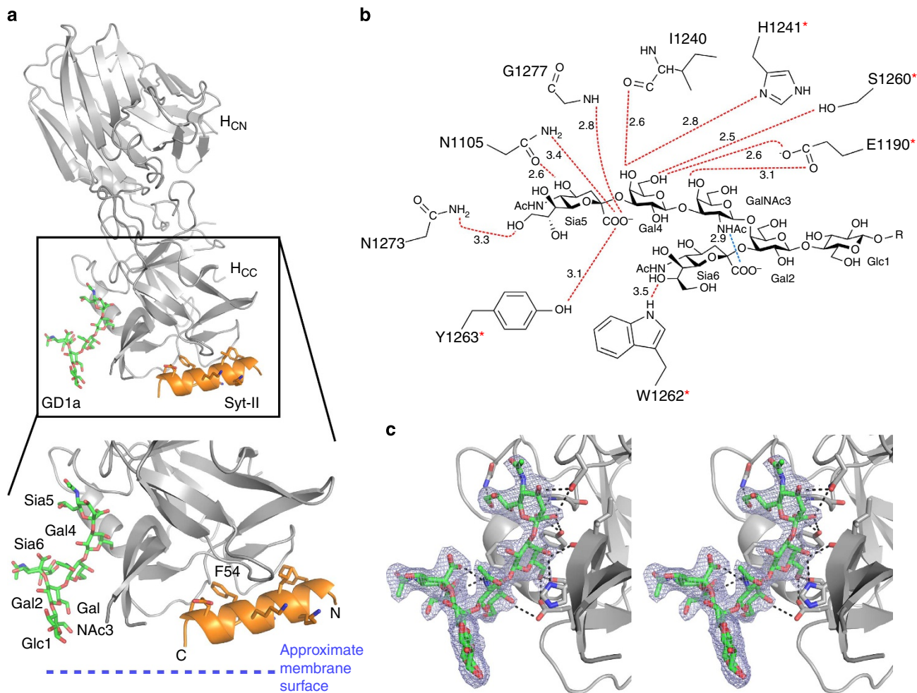
Figure 1 | Dual receptor binding to BoNT/B. (a) Overall view of BoNT/B (grey) with GD1a (green) and mouse Syt-II (orange) bound. Lower panel shows a close-up view on the GD1a- and Syt-II-binding sites, with the GD1a moieties and the Syt-II residues, interacting with BoNT/B, shown as sticks. Phenylalanine 54 is indicated, this position is a leucine in human Syt-II that has a drastically lower affinity to BoNT/B than mouse Syt-II 17,44 . (b) Schematic overview of possible hydrogen bonds between GD1a and BoNT/B (red dashed lines) and an internal hydrogen bond (blue dashed line). The hydrogen bond distance is shown for each bond (Å). Red stars show residues that previously, via mutagenesis, have been shown to be important for ganglioside binding 26 . In GD1a, a ceramide is present at the R position, the GD1a oligosaccharide used here has a hydrogen in this position. (c) Stereo view of the bound GD1a, with its electron density ( 2F_o - F_c map contoured at 1.5\sigma ) in blue, and the possible hydrogen bonds to BoNT/B residues as dashed lines.
