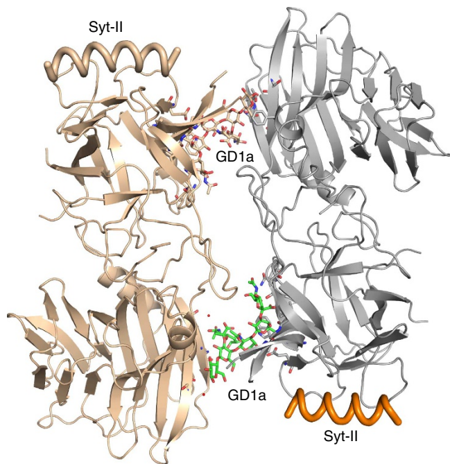
Figure 3 | The asymmetric unit. The asymmetric unit containing two molecules of BoNT/B (grey), with the bound recognition domain of Syt-II (orange) and GD1a (green). The second copy of each molecule is coloured in beige. All residues that interact with GD1a are shown as sticks. Crystal contacts are formed between the two BoNT/B protomers (grey and beige) in the asymmetric unit via the bound GD1a molecules. GD1a is bound to the GBS, as described in Fig. 1. The crystal contacts are formed by Glc1, Gal2 and Sia6. The green GD1a forms three hydrogen bonds, to S984, N1025 and L1022. The beige GD1a forms five hydrogen bonds to S984, F986, N1025 and T1026. These interactions are not biologically relevant, as BoNT/B has been shown to have a single GBS 26 .
