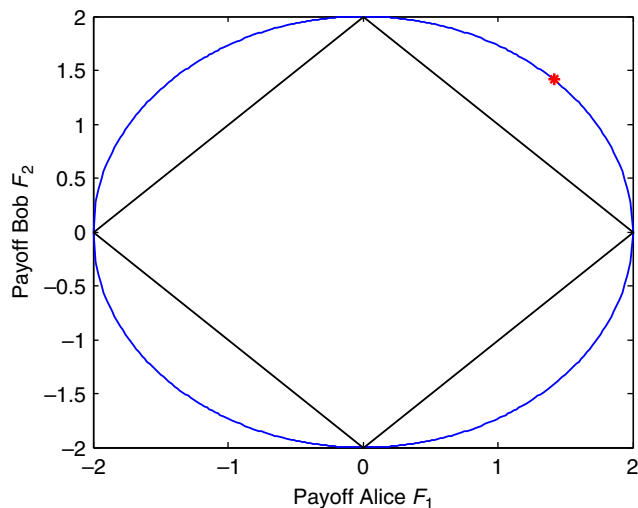
Figure 2 | Space of possible average payoffs functions. The pairs of payoffs achievable with classical advice are represented by the back polytope (square). Players sharing quantum advice have access to a strictly larger set of possible payoff function (blue circle), and hence have an advantage over classical players. The red star represents the particular quantum strategy mentioned in the main text. Players having access to super-quantum advice can reach all points, in particular the point F_1 = F_2 = 2 , a no-signalling Nash equilibrium.
