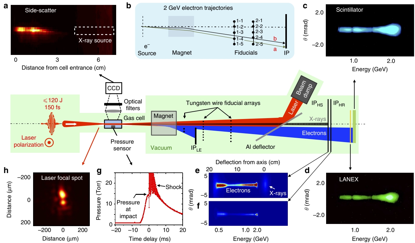
Figure 1 | Schematic diagram of PW laser-driven wakefield accelerator. The main components were enclosed in a vacuum chamber, highlighted in green, which was kept at 10^{-6} Torr. The PW laser pulse, entering from the left and linearly polarized perpendicular to the plane of the drawing, was focused into the gas cell, where it created a He plasma and wake that captured and accelerated electrons to 2 GeV. Electrons and betatron X-rays emerging from the cell exit aperture passed through a magnetic field, then through two linear arrays of eight 127\ \mu\text{m} diameter tungsten-wire fiducials located 1.256 and 1.764 m, respectively, downstream from the cell exit. A 25\text{-}\mu\text{m} thick Al foil deflected the transmitted laser pulse to a beam dump. Undelected X-rays and energy-dispersed electrons above 0.5 GeV passed through this foil, and exposed in sequence a high-sensitivity (HS) imaging plate ( \text{IP}_{\text{HS}} ), a high-resolution (HR) IP ( \text{IP}_{\text{HR}} ), a phosphorescing screen (LANEX) and a plastic scintillator. An additional \text{IP}_{\text{LE}} recorded low-energy (LE) electrons ( <0.35 GeV) after they passed through a third array of fiducials. Surrounding panels highlight various diagnostics and details, clockwise from upper left: (a) transversely scattered light, spectrally filtered and imaged to a CCD camera (the dashed rectangle shows the region near the cell exit from which betatron X-rays originated, as determined by X-ray triangulation); (b) trajectories of 2 GeV electrons for shots that yielded the results in Fig. 2a,b (labelled 'a' and 'b', respectively) relative to the fiducial arrays (labelled 1-1 through to 1-8 for the first array and 2-1 through to 2-8 for the second array); (c-f) , unprocessed data showing electrons up to 2.3 GeV and fiducial shadows for the shot that yielded the results in Fig. 2a, as detected on (c) scintillator, (d) LANEX, (e) \text{IP}_{\text{HS}} (also showing undeflected X-rays) and (f) \text{IP}_{\text{HR}} ; (g) He pressure versus time, and an acoustic shock when the laser pulse arrived, as recorded by a fast pressure transducer; (h) a typical laser focal spot.
