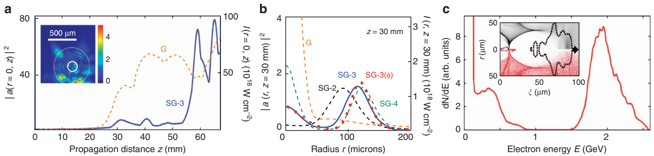
Figure 4 | WAKE simulation results. Initial conditions are: pre-ionized plasma of density n_e = 5.0 \times 10^{17} \text{ cm}^{-3} ; incident laser pulse of duration \tau = 160 \text{ fs} , energy = 100 J (peak laser strength parameter a_0 = 0.58 , normalized power P/P_{cr} = 20 ). (a) Laser strength parameter a(r=0, z) and peak intensity I(r=0, z) along propagation axis inside plasma for initially Gaussian (G, dashed orange line) and third-order super-Gaussian (SG-3, solid blue) pulses of radius w_0 = 275 \mu\text{m} , the latter showing two rapid self-focus/defocus cycles near the cell exit. Inset: image of incident laser profile at approximately the cell entrance, \sim 2 \text{ cm} from its focal plane, for shot ‘a’ in Fig. 2, compared with white dashed circle of radius w_0 = 275 \mu\text{m} and white solid circle of radius w_0 = 80 \mu\text{m} . Colour scale indicates intensity as a multiple of 10^{17} \text{ W cm}^{-2} . (b) Transverse profiles at z = 30 \text{ mm} of initially Gaussian (G, short-dashed orange), second- (SG-2, short-dashed black), third- (SG-3, solid blue) and fourth- (SG-4, long-dashed green) order super-Gaussian pulses, showing Airy-ring-like structure for non-Gaussian profiles that is evidently critical for self injection. Each profile is plotted for the longitudinal position of maximum \int_0^\infty r dr I(r) within the pump profile; this position differs slightly for each plot, and from the position of maximum peak intensity shown in a . For comparison, curve SG-3( \phi ) (red squares) shows the transverse profile at z = 30 \text{ mm} , calculated with the NLSE, of an initially third-order super-Gaussian multiplied by the azimuthally varying function 1 + 0.25(r/w_0)^9 \cos(9\phi) to mimic an evolving array of hotspots. (c) Simulated electron energy spectrum at z = 6.8 \text{ cm} for initially third-order super-Gaussian pulse evolving as in a , showing 2 GeV peak and low-energy tail. Similar spectra were obtained for other super-Gaussian orders and for \pm 10\% variations in a_0 . Inset: electron density profile, showing background plasma electrons (black, top) and test electrons (red, bottom). Injected electrons are the red feature inside evacuated bubble. \zeta denotes longitudinal distance along the bubble’s axis. Black dashed curve: 8 \times 10^{18} \text{ W cm}^{-2} iso-intensity contour of laser pulse at z = 6.8 \text{ cm} .
