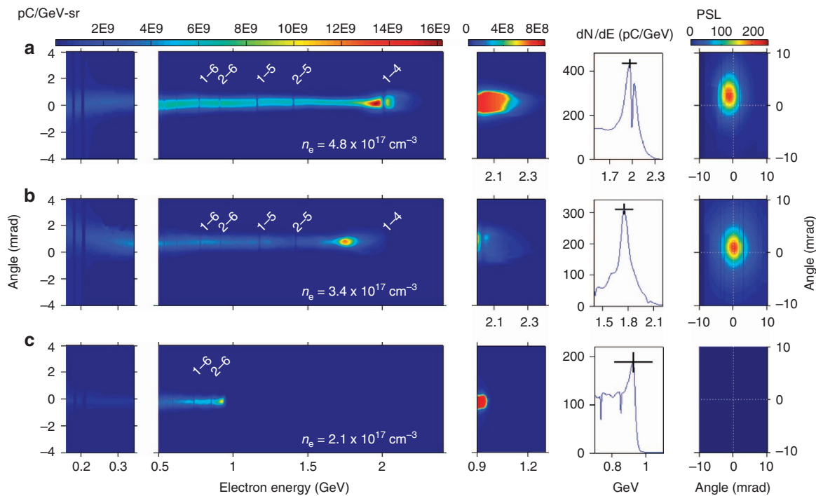
Figure 2 | Electron spectra and betatron X-ray profiles for three shots from the accelerator. First column: sub-GeV electron spectra recorded on IP_{LE} ; second column: GeV electron spectra recorded on IP_{HS} ; third column: detail of high-energy tails; fourth column: vertically integrated spectra around each high-energy peak; fifth column: betatron X-ray angular distribution recorded on IP_{HS} . (a) Results for shot yielding quasi-monoenergetic peak at 2.0 GeV, with n_e = 4.8 \times 10^{17} \text{ cm}^{-3} , obtained from raw data shown in Fig. 1e. Results for (b) n_e = 3.4 \times 10^{17} \text{ cm}^{-3} , yielding peak at 1.8 GeV, and (c) n_e = 2.1 \times 10^{17} \text{ cm}^{-3} , yielding peak at 0.95 GeV. Table 1 lists complete laser-plasma conditions and e-beam properties for each shot. Fiducial wire shadows are labelled as in Fig. 1b. On each vertical scale, ‘0 mrad’ denotes the average vertical position of a 30-shot sequence of GeV electrons. In the fourth column, vertical error bars represent the average uncertainty in the calibration of each of IP_{HS} , high-resolution IP ( IP_{HR} ) and LANEX as charge monitors ( \pm 10\% ); horizontal error bars represent 2\sigma uncertainty in the peak position, derived from the uncertainty in fitting the calculated trajectories of electrons near 2 GeV to the observed positions of fiducial shadows on IP_{HS} for each shot. This uncertainty originates in turn from the combined uncertainty in fiducial wire positions ( \pm 25 \mu\text{m} transversely, \pm 2 \text{ mm} longitudinally), fiducial shadow positions ( \pm 1/2 pixel, or \pm 50 \mu\text{m} ), electron source position (determined by X-ray triangulation) relative to magnet and detector ( \pm 75 \mu\text{m} transversely, \pm 1 \text{ cm} longitudinally) and magnetic field ( \pm 1\% ).
