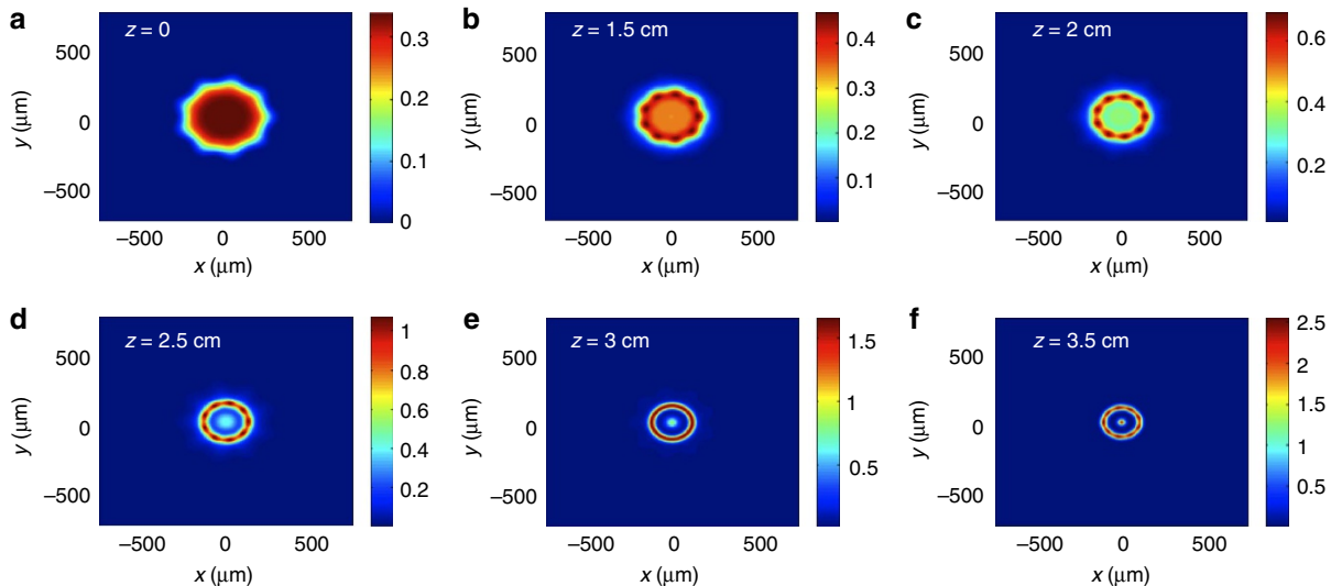
Figure 5 | NLSE simulation illustrating topological changes of a relativistically self-focusing laser pulse. The colour bars indicate the squared laser strength parameter a^2 . The laser pulse evolves according to the NLSE in a plasma of density n_e = 5 \times 10^{17} \text{ cm}^{-3} . (a) Initial pulse at z = 0 with azimuthally modulated super-Gaussian profile. Algebraic form and parameters are given in Methods. (b,c) The azimuthal perturbations quickly evolve into distinct hotspots by z = 2 \text{ cm} , similar to those present in the actual laser pulse. (d,e) Hotspots then evolve into a nearly cylindrically symmetric ring by z = 3 \text{ cm} , as the central peak intensifies. At this point, the radial profile is very similar to that of initially cylindrically symmetric super-Gaussian pulses, as shown in Fig. 4b. (f) By z = 3.5 \text{ cm} , the central peak becomes more intense than the outer ring. WAKE simulations of similar profiles suggest that this central peak continues intensifying rapidly, eventually forming a rapidly evolving bubble into which surrounding plasma electrons inject. At z = 3.5 \text{ cm} , however, the density perturbation has already become substantial, invalidating further description by the NLSE.
