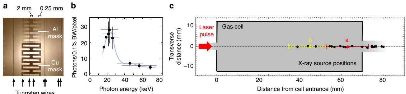
Figure 3 | Betatron X-ray data. (a) Typical radiograph of Al and Cu masks backlit by betatron X-rays from the accelerator recorded on IP HS . Masks vary in thickness in four lateral steps: 2 mm (centre), 1 mm, 0.5 mm and 0.25 mm (edge). Vertical lines are shadows of tungsten-wire fiducials. (b) Typical X-ray spectrum. Data points were obtained by analysing transmittance of the Cu/Al masks (see Methods). Horizontal error bars correspond to the FWHM of the f_k distribution (see Methods); vertical error bars represent uncertainty in X-ray transmission caused by scattering at edges of the filter masks, and error in reconstructing the incident X-ray intensity profile from transmission through gaps in the masks. Blue curve is a cubic spline fit to the data points. (c) X-ray source locations within the 7 cm gas cell for 22 shots that yielded >1 GeV electrons, determined by triangulation from tungsten-wire fiducial shadows. Source locations for shots in Fig. 2a,b are labelled 'a' (red) and 'b' (yellow), respectively. Horizontal error bars ( \pm 10 mm) indicate triangulation error arising from uncertainty in measuring fiducial wire positions.
