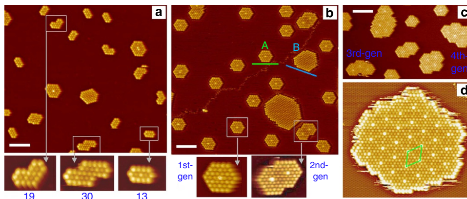
Figure 1 | C_{60} islands with unusual shapes and magic sizes. (a) Immediately after warming up a sample (0.1 ML of C_{60} ) prepared at 115 K to RT, small (10–30 of C_{60} ) ordered islands with non-compact shapes such as boomerang (19-mer), zigzag (30-mer) and stadium (13-mer) are formed. (b) After annealing the sample (0.2 ML of C_{60} ) at RT for 2 h, medium-size islands with compact shapes appear. Most islands have the shape of a hexagon or two overlapped hexagons, each possessing a characteristic central bright spot, which is used as an indicator of an island's generation. The green and blue lines show lattice orientations of the A- and B-phase islands, respectively. (c) Deposition of higher coverage of C_{60} at RT leads to the formation of larger islands with characteristic shape of overlapped hexagons. (d) A large island formed by deposition of C_{60} at RT exhibits moiré interference pattern with similar characteristic periodical bright spots. The green rhombus indicates the unit cell of the moiré pattern. Scale bar, 10 nm (a–c).
