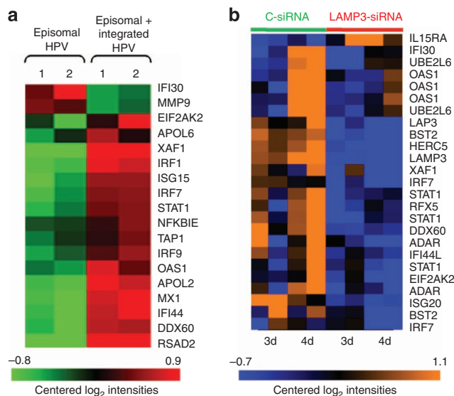
Figure 6 | Antiviral subnetwork genes are regulated by LAMP3.
