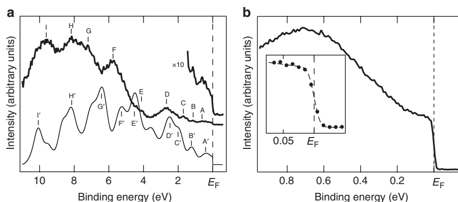
Figure 2 | Angle-integrated results and first-principles calculations. Angle-integrated photoemission spectra of (BEDT-TTF) 3 Br(pBIB) measured at 4 K using the photon source of (a) He I \alpha (bold line), plotted along with first-principles band structure calculations broadened by convolving with a Gaussian corresponding to the experimental energy resolution (thin line). Labels A–I and A'–I' mark features in the experimental spectrum and first-principles band calculations, respectively. (b) The laser-PES data measured for (BEDT-TTF) 3 Br(pBIB) up to a binding energy of 1 eV below the Fermi level (solid line). Inset shows the spectrum near E_F indicating the existence of a metallic Fermi edge (circle), which can be well reproduced by a Fermi-Dirac function convolved with a Gaussian corresponding to the experimental energy resolution (broken line).
