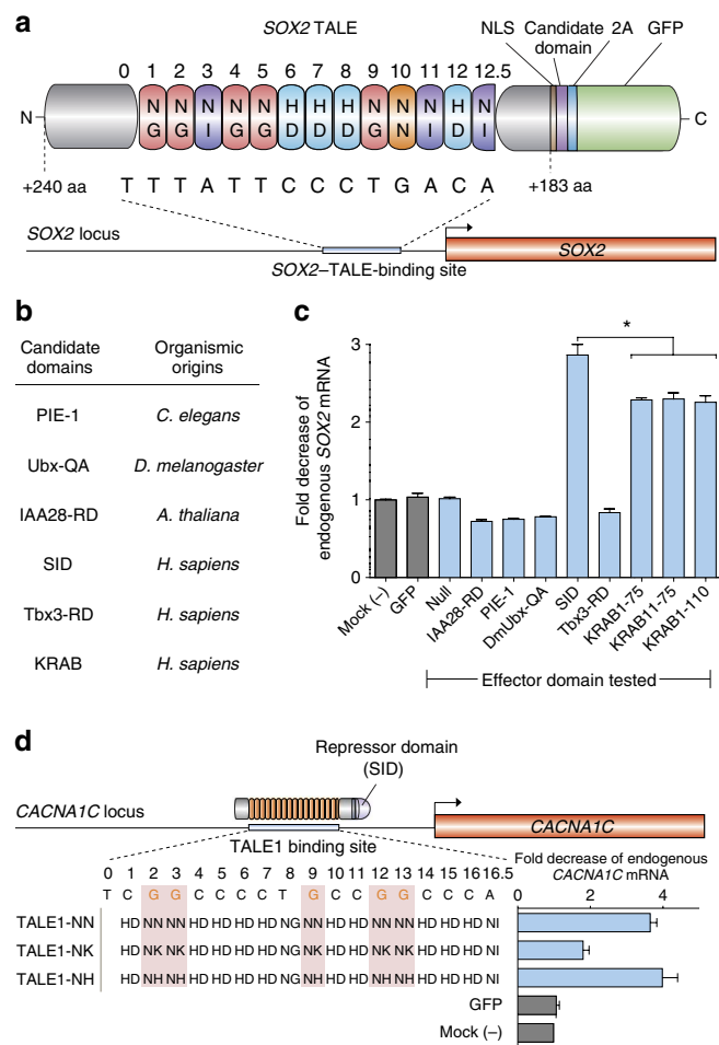
Figure 4 | Development of aTALE transcriptional repressor architecture. (a) Design of SOX2 TALE for TALE-repressor screening. A TALE targeting a 14-bp sequence within the SOX2 locus of the human genome was synthesized as described previously 3 . (b) List of all repressors screened and their host origin (left). Eight different candidate repressor domains were fused to the C-term of the SOX2 TALE. (c) The fold decrease of endogenous SOX2 messenger RNA (mRNA) is measured using qRT-PCR by dividing the SOX2 mRNA levels in mock-transfected cells by SOX2 mRNA levels in cells transfected with each candidate TALE repressor. (d) Transcriptional repression of endogenous CACNA1C. TALEs using NN, NK and NH as the G-targeting RVD were constructed to target a 18-bp target site within the human CACNA1C locus (site 1 in Fig. 3). Each TALE is fused to the SID repression domain. NLS, nuclear localization signal; KRAB, Krüppel-associated box. All results are collected from three independent experiments in HEK 293FT cells. Error bars indicate s.e.m.; n = 3 . * P < 0.05 , Student's t -test.
