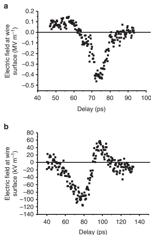
Figure 4 | Electric field of the SPP at the surface of the wire as a function of time. (a) Measurements of the field strength on the wire surface taken at the position z = 80 mm from the tip of the wire. For each setting of the time delay between the probe pulse and the laser pulse used for photoemission of the electron bunch, the electric field strength at the surface of the wire was extracted from images recorded in the same manner as Fig. 3. (b) Field strengths measured after the bend in the wire (33 mm radius of curvature) using a balanced diode set-up instead of the double-CCD camera used in (a). Zero delay is arbitrary for both (a,b).
