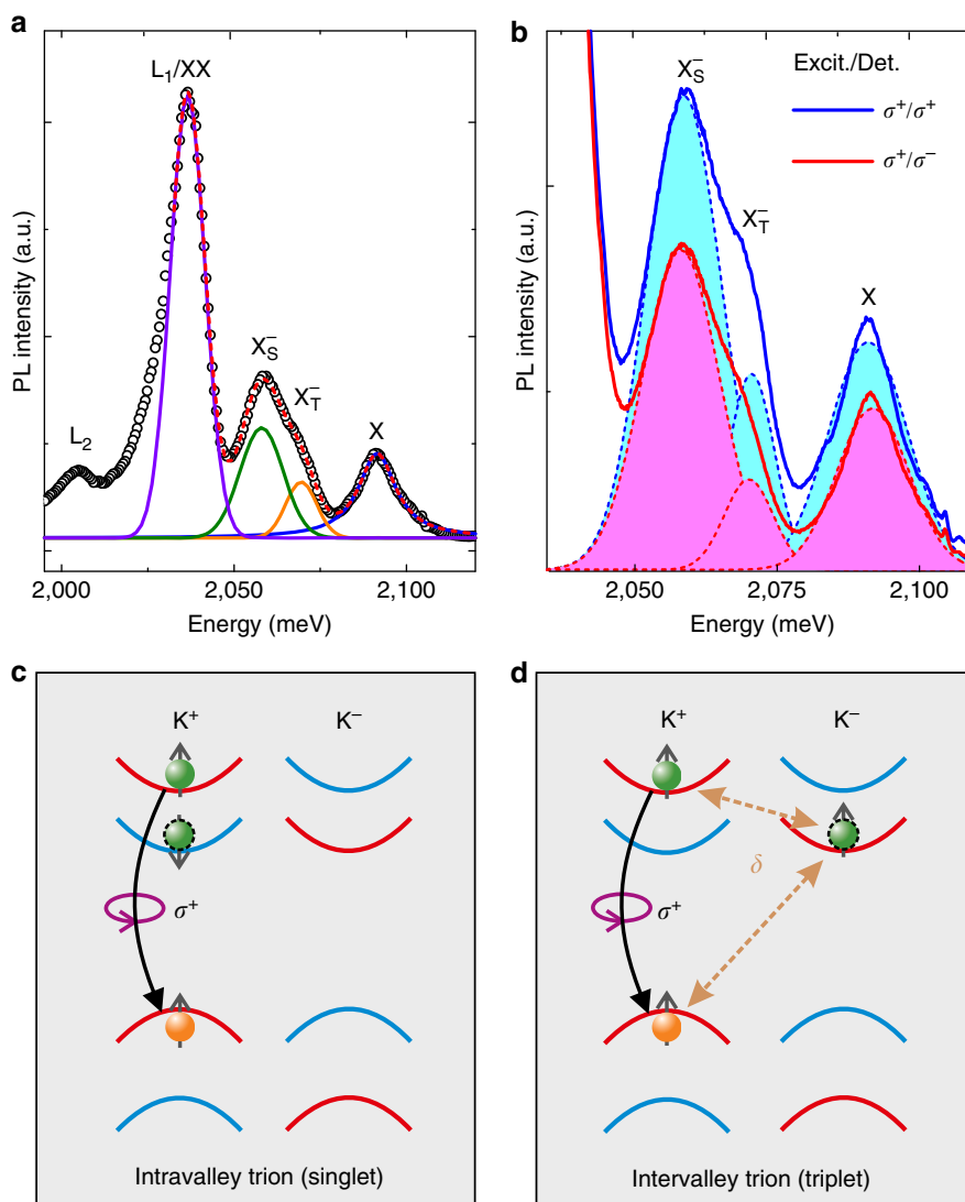
Figure 1 | Trion fine structure and valley polarization observed in low-temperature PL. (a) PL spectrum of monolayer WS 2 at a temperature of 4 K. The black circles represent the data, the red curve is the sum of the fit functions for neutral A excitons X (blue), the peaks we associate with triplet X T - (orange) and singlet trions X S - (green), and the biexciton/localized exciton complex XX/L 1 (violet). In addition, a second localized exciton peak L 2 at lower energies is visible. (b) Helicity-resolved PL spectra of the same flake as depicted in (a). The solid blue (red) lines represent the data for co-(contra-)circular excitation (Excit.) and detection (Det.), the dashed lines in corresponding colours are fit functions for X, X T - and X S - . Circular polarization degrees of the different excitonic features are calculated by evaluating the areas under the corresponding fit curves. (c,d) Schematic illustration of singlet (c) and triplet (d) trion configurations for WS 2 in the K + valley. Electrons in the conduction (valence) band are represented by green (orange) spheres. Spin-up (-down) bands appear in red (blue) colour. The curved arrows indicate the interband recombination. The final state of the remaining conduction-band electron after trion recombination is marked by the dashed black outline. The intervalley electron-hole exchange interaction leading to an energetic splitting \delta is indicated by the dashed arrows.
