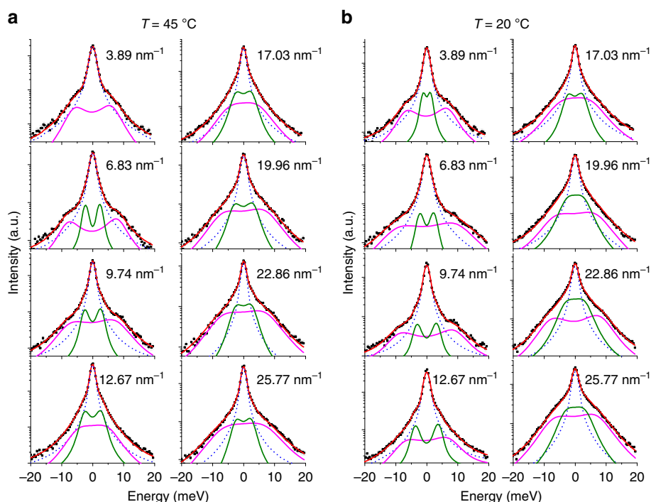
Figure 2 | IXS spectra of DPPC. (a) IXS spectra measured at T=45^\circ\text{C} in the fluid phase and at (b) T=20^\circ\text{C} in the gel phase. The experimental data (black squares) with error bars signifying 1 s.d. are reported together with the best least squares fit (red solid curves) using a DHO model with two excitations. The DHO models are presented after convolution with the IXS spectrometer RF (denoted by the dashed blue line). Low- and high-frequency DHO are denoted by the green and magenta solid curves, respectively. The corresponding Q values are shown in each plot.
