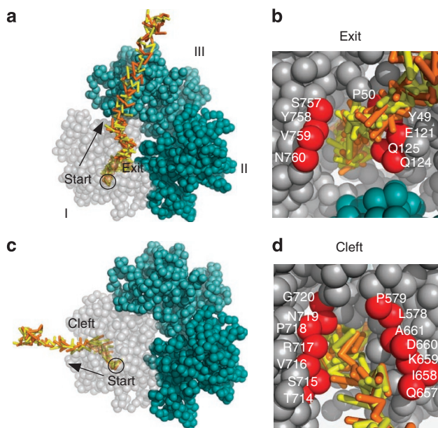
Figure 4 | Snapshots of drug export through 'exit' and 'cleft'. The snapshots of the drug in an exporting process are superimposed, and the odd and even time slices are in yellow and orange respectively. The protomer I is drawn transparent. The circle and arrow indicate the starting point and the direction of export respectively. (a) The drug was exported through 'exit'. (b) Closed-up view of the 'exit'; some residues are labelled and drawn in red. (c) and (d) show the drug export through the 'cleft' and the closed-up view of the 'cleft' respectively.
