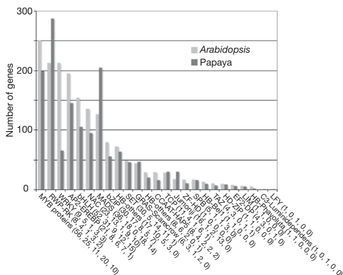
Figure 2 | Comparison of gene numbers in transcription-factor tribe or related tribes from Arabidopsis and papaya. Most transcription factors are represented by fewer genes in papaya than Arabidopsis . Transcription-factor names are given, with values after the names corresponding to: number of tribes with genes assigned to transcription factor group, number of tribes with smaller counts in papaya than Arabidopsis , number of tribes with equal counts in papaya and Arabidopsis , number of tribes with larger counts in papaya, and number of tribes with zero members in papaya. Supporting data are provided in Supplementary Table 8.
