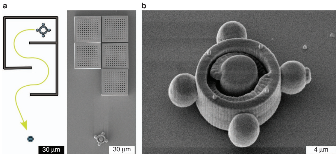
Figure 5 (a) Schematic depiction of the maze-like compartment. Using optical forces, the nut can be guided outside and assembled with the fixed screw. (b) The SEM image shows a stable screw connection of the microcomponents.
