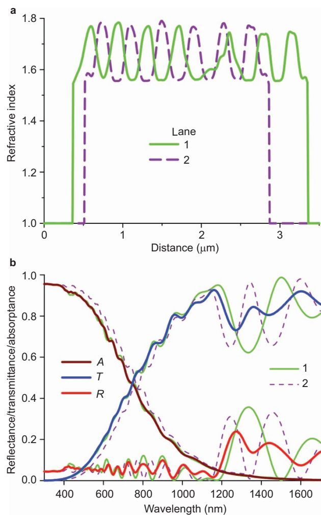
Figure 4 Refractive index profiles and their spectral consequences. (a) The real part of the refractive index at 500 nm for the two 0.5 \mu\text{m} wide lanes numbered 1 and 2 in Figure 2f. (b) Absorptance (A), transmittance (T) and reflectance (R) spectra for normally incident light, calculated with a multilayer model for lanes 1 and 2 and the averaged spectra (brown, blue and red curves, respectively).
