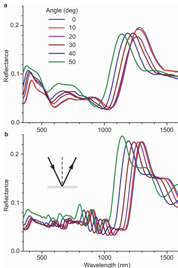
Figure 5 Angle-dependent reflectance spectra. (a) Averaged spectra calculated for 36 lanes of the transmission electron micrograph of Figure 2f, for angles of incidence 0°–50°. (b) Reflectance spectra measured for each angle of incidence at the mirror angle.
