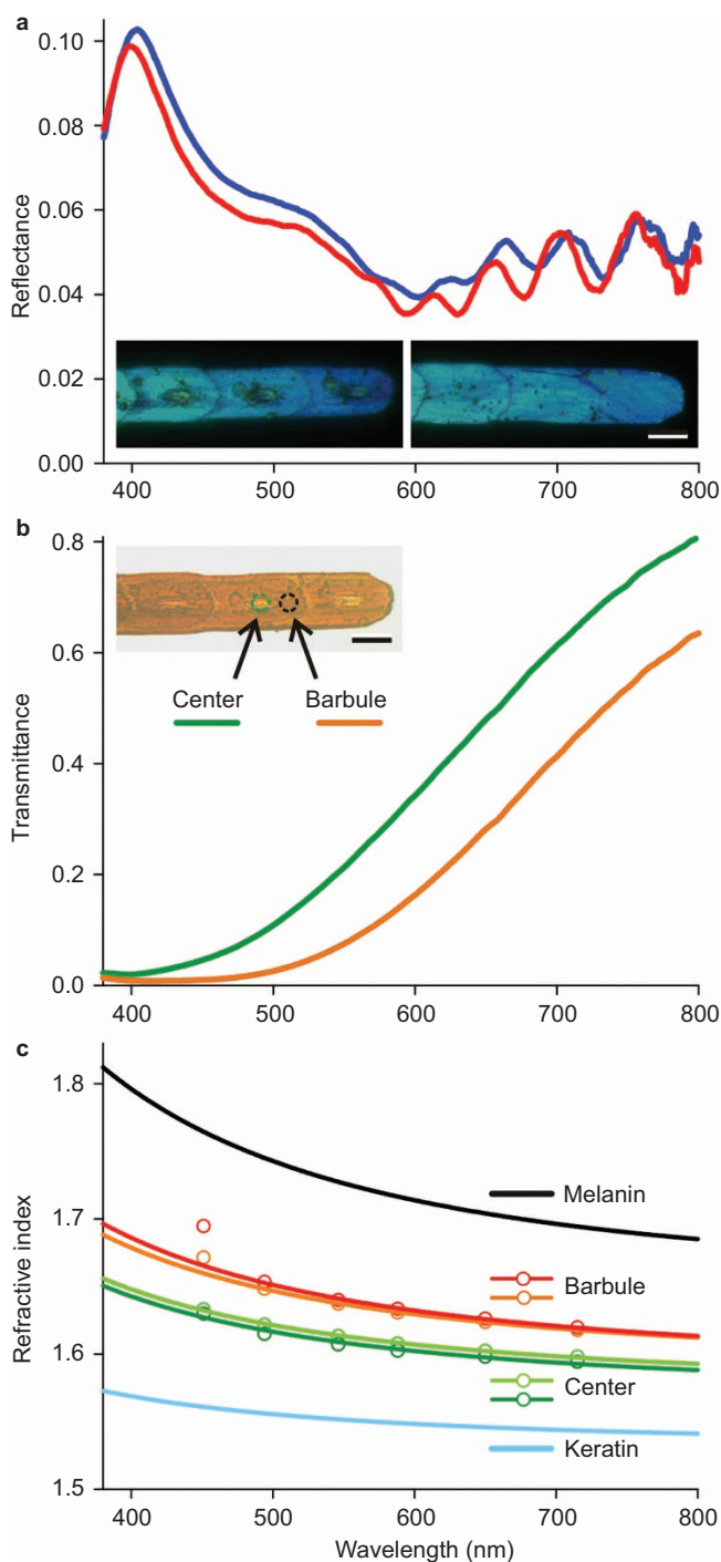
Figure 3 Reflectance, transmittance and refractive index of occipital feather barbules. (a) Reflectance spectra measured from small barbule areas ( \sim 5 \mu\text{m} diameter, upperside) showing oscillations reminiscent of thin film interference. Insets: a barbule observed with epi-illumination from the underside (left) and upperside (right; scale bar: 20 \mu\text{m} ). (b) Transmittance spectra measured from the center of a barbule cell and from an area outside the center. Inset: the same barbule as that in a observed with transmitted light (scale bar: 20 \mu\text{m} ). (c) Refractive index of barbule and center areas as a function of wavelength, derived from Jamin-Lebedeff interference microscopy, with Cauchy function fits, together with the refractive index of bird keratin 11 and the derived melanin refractive index.
