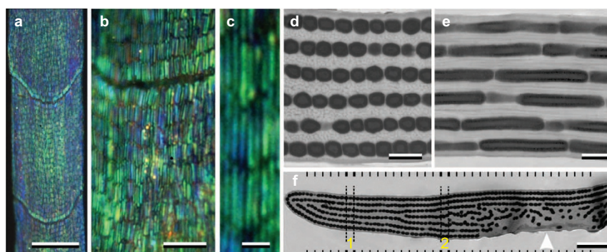
Figure 2 Anatomy of the distal barbules of the occipital feathers. (a) A single barbule immersed in a fluid with refractive index 1.63 (at 589 nm) observed with epi-illumination light microscopy. The barbule consists of a row of cells. (b) At higher magnification, individual melanin rodlets can be discerned. (c) Close-up view showing the single melanin rodlets, parallel arranged in bands. (d) Transmission electron micrograph of a cross-section, revealing ordered layers of rodlets, diameter \sim 250 nm, showing a \sim 60 nm thick cladding with a slightly higher electron density than the core. (e) Longitudinal section of the rodlets. (f) A cross-section perpendicular to the barbule axis. The layered order of the rodlets is distorted in a central area at the underside (arrowhead). The short vertical bars indicate 36 vertical lanes, 0.5 \mu\text{m} wide, for which reflectance, transmittance and absorbance spectra were calculated. For the two lanes flanked by bold bars (numbered 1 and 2 and marked by dotted border lines), calculated refractive index profiles and spectra are given in Figure 4. Scale bars: a 20 \mu\text{m} ; b 5 \mu\text{m} ; c 1 \mu\text{m} ; d, e 0.5 \mu\text{m} ; f 2 \mu\text{m} .
