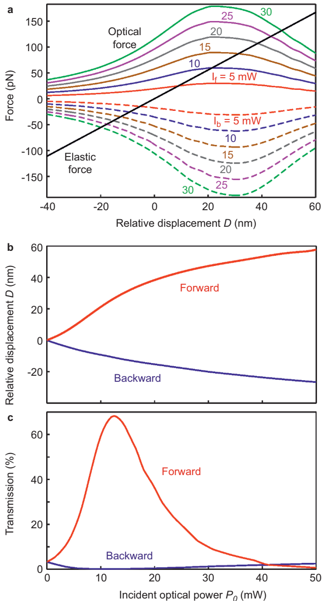
Figure 2 Nonlinear optical response and asymmetric transmission. (a) Dependence of the relative optical force F_{opt}^{beam} on the mutual out-of-plane displacement D of neighboring silicon nitride beams supporting thick and thin silicon nano-bars under 1551 nm forward (solid lines) and backward (dashed lines) illumination at a range of incident power levels P_0 (as labeled). The straight black line corresponds to the opposing elastic force. (b, c) Dependencies of (b) relative nano-beam displacement and (c) metamaterial optical transmission on total incident power at a wavelength of 1551 nm ( D = D_2 - D_1 where D_1 and D_2 are the absolute displacements of beams supporting thick and thin Si nano-bars respectively).
