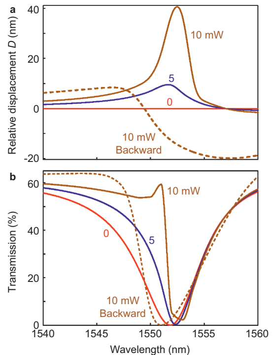
Figure 3 Optomechanical nonlinearity and asymmetric transmission resonances. (a) Spectral dispersion of the steady-state relative nano-beam displacement and (b) corresponding optical transmission for forward incidence of light (solid lines) at a selection of total incident power levels (as labeled) and backward incidence at 10 mW (dashed lines).
