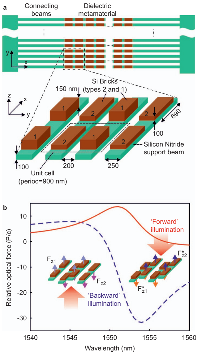
Figure 1 Asymmetric optomechanical forces in a dielectric photonic metamaterial. (a) Artistic impression and dimensional details of the parallel silicon nitride beam, silicon nano-bar metamaterial configuration studied. (b) Spectral dispersion of the relative optical force F_{\text{opt}}^{\text{cell}} on the two nanobar elements of a single metamaterial unit cell under normally incident x -polarized illumination for both forward ( -z ) and backward ( +z ) directions of light propagation ( F_{\text{opt}}^{\text{cell}} = F_{z2} - F_{z1} , where F_{z1} and F_{z2} are the optical forces on the thick and thin bars, respectively; Optical force is presented in units of P/c , where P is the incident power per unit cell and c is the speed of light in vacuum).
