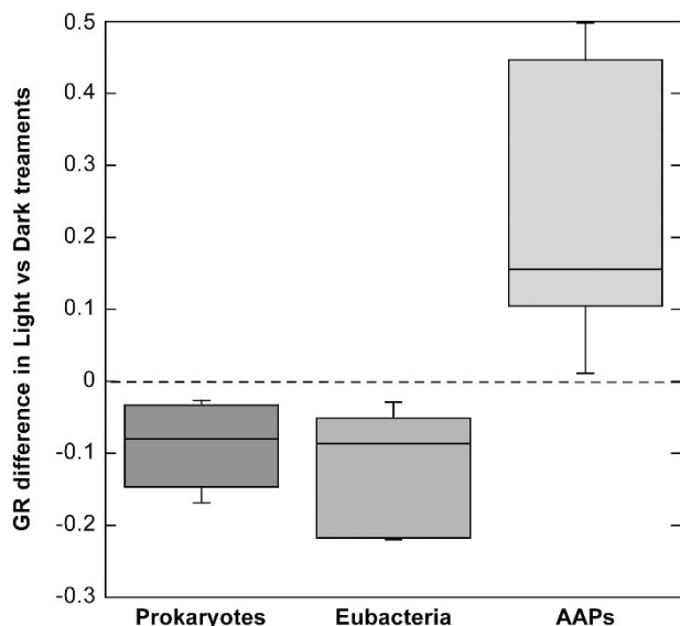
Figure 2 Box plots showing the distribution of the difference between growth rates (GR) in the light and dark treatments (positive values indicate higher growth rates in the light and vice versa) for the microbial groups studied. Values from all treatments and experiments are pooled. From top to bottom, the horizontal lines of the box represent the upper-quartile, median and lower-quartile. Whiskers extending from top and bottom of the box represent maximum and minimum values. AAP, aerobic anoxygenic phototrophic bacteria; EUB, Eubacteria ; PRO, total prokaryotes.
