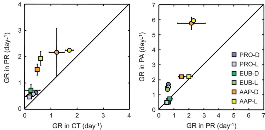
Figure 1 Growth rates in the predator-reduced (PR) vs the control (CT) treatments (left panel) and in the phosphorus-amended (PA) vs the PR treatments (right panel). Circles correspond to Experiment 1 and squares to Experiment 2. Dots falling on the 1:1 line indicate that growth rates have the same value for both x-y treatments; if dots are above or below the line, growth rates from y treatments are higher or lower than in x treatments respectively. Error bars represent the standard deviations. AAP, aerobic anoxyphototrophic bacteria; D, Dark incubations; EUB, Eubacteria ; L, Light-dark incubations; PRO, total prokaryotes.
