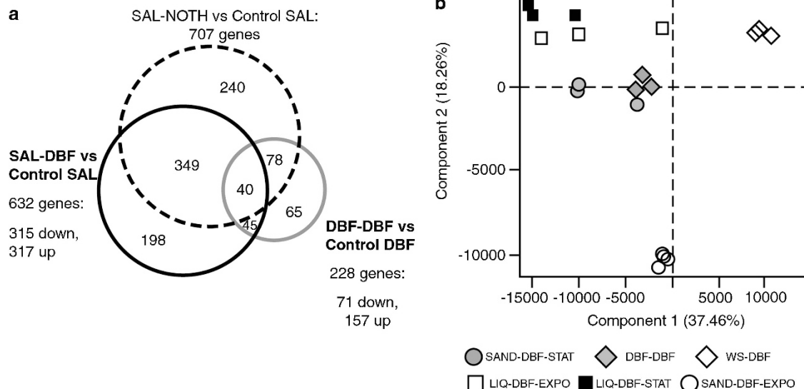
Figure 3 Group clustering of transcriptome data. (a) Venn diagram of the numbers of differentially expressed RW1 genes in pair-wise comparisons between 1-h treatments. SAL-NOTH , cells inoculated in bare sand from salicylate cultures; SAL-DBF , cells from salicylate cultures inoculated in sand contaminated with DBF; DBF-DBF , cells from DBF liquid cultures inoculated in sand contaminated with DBF. (b) Two-dimensional Principal Component Analysis of Spingomonas wittichii transcriptomes under different growth conditions. Global patterns of RW1 cells growing in sand in exponential (SAND-DBF-EXPO) or stationary phase (SAND-DBF-STAT) vs liquid cultures with crystals of dibenzofuran in exponential (LIQ-DBF-EXPO) or stationary phase (LIQ-DBF-STAT). DBF-DBF, transcriptome from cells grown on DBF inoculated during 1 h in sand with DBF. WS-DBF exponential growth in liquid with saturated amounts of DBF (WS-DBF).
