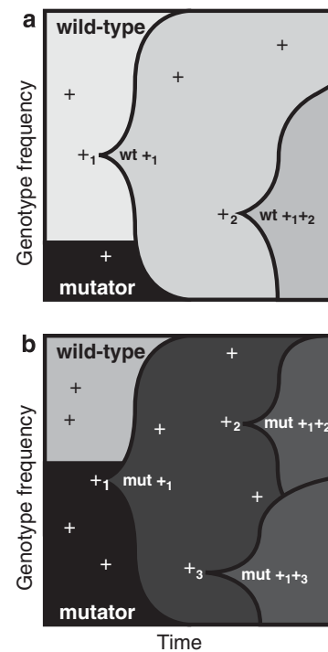
Figure 1 Mutator hitchhiking depends on the relative mutation supply rates to mutator and wild-type subpopulations. (a) When a mutator allele is rare, the subpopulation with the wild-type mutation rate can have a higher mutation supply rate than the mutator subpopulation and therefore will tend to acquire new beneficial mutations more quickly. This keeps the mutator from rising in frequency. (b) If sufficiently common, a mutator subpopulation can have a higher mutation supply rate than the wild type. Each new beneficial mutation then has a higher tendency to arise in association with the mutator, causing the mutator to hitchhike toward higher frequency.
