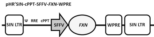
Figure 8. Schematic representation of pHR'SIN-cPPT-SFFV-FXN-WPRE. The pHR'SIN-cPPT-SFFV-FXN-WPRE vector is self-inactivating (SIN) configuration with a WPRE and an internal spleen focus-forming virus promoter-driving FXN gene expression. VSV-G pseudotyped pHR'SIN-cPPT-SFFV-FXN-WPRE was generated by HEK293T cells to a titer of 1 \times 10^8 TU ml -1 for infecting FRDA fibroblasts.
