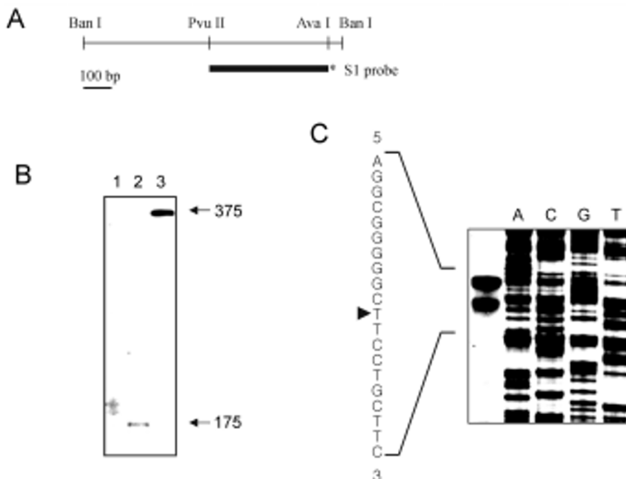
Figure 2. Identification of the transcription start site of the human PLC-β2 gene. A. The restriction map of pB2B5. B. S1 nuclease mapping analysis. PvuII / Aval fragment described in A was used as a probe. Lane 1, control products with yeast tRNA, lane 2, the protected fragments with Daudi RNA, lane 3, the S1 probe. Protected fragments containing 175 bases are indicated by arrow. C. Primer extension analysis, 32 P-labeled oligo A was hybridized to 50 μg of total RNA from Daudi cells. The dideoxy-sequencing ladder of the same strand is shown. The arrowhead indicates a putative major transcription start site.
