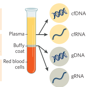
Fig. 2 | Caris' liquid-biopsy platform, Caris Assure, provides a comprehensive and non-invasive approach to profiling. bTMB, blood tumor mutational burden; cfDNA, cell-free DNA; cfRNA, cell-free RNA; CHIP, clonal hematopoiesis of indeterminate potential; gDNA, genomic DNA; gLOH, genome-wide loss of heterozygosity; gRNA, genomic RNA; MSI, microsatellite instability; WES, whole-exome DNA sequencing; WTS, whole-transcriptome RNA sequencing.
