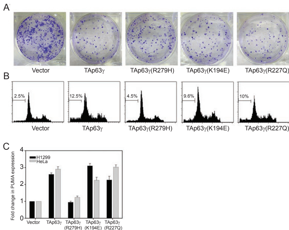
Figure 7 Effect of TAp63 \gamma mutants on cell growth. H1299 cells were transfected with either TAp63 \gamma or representative TAp63 \gamma mutants or empty vector control as indicated. (A) The colonies stained with crystal violet from a representative experiment are shown. (B) H1299 cells were co-transfected with either TAp63 \gamma mutants or wild TAp63 \gamma and membrane-bound hybrid-US9GFP (PAB35). Cells were harvested at 48 h post-transfection, fixed in 70% ethanol and DNA stained with propidium iodide solution, as described in Materials and Methods. DNA distribution was analyzed using flow cytometry using CellQuest Program. The histogram represents the percentage of sub-G1 cells positive for PI and membrane-bound hybrid GFP. (C) Total RNA was extracted and TaqMan-based real-time PCR analysis was performed to detect the transcript levels of PUMA. The Y-axis represents the fold change in PUMA transcript levels relative to vector-transfected cells.
