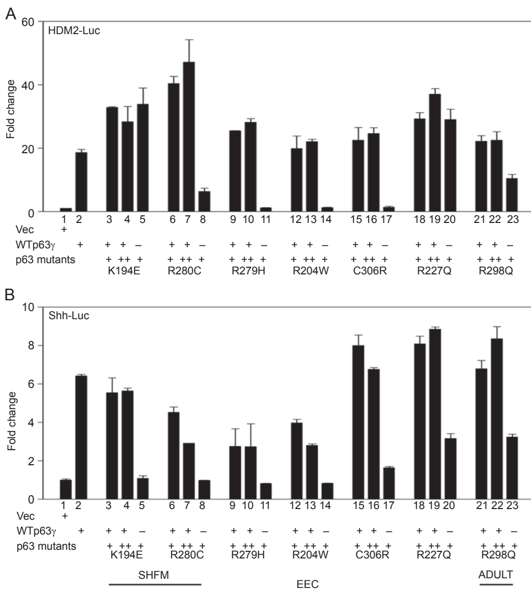
Figure 3 TAp63γ mutants differentially affect the wildtype-TAp63γ-mediated transactivation. H1299 cells were transfected with the Hdm2-Luc (A) or Shh-Luc reporter (B) alone or co-transfected with wildtype TAp63γ alone or along with TAp63γ mutants as indicated using lipofectamine 2000. The Y-axis represents the fold change in relative luciferase units compared with empty vector.
