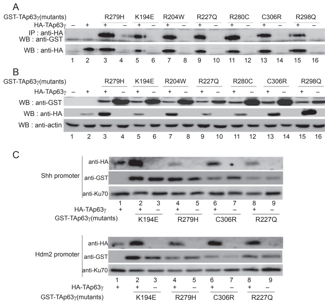
Figure 6 TAp63 \gamma mutants interact with wildtype TAp63 \gamma and affect its DNA-binding activity. H1299 cells were transfected with HA-tagged TAp63 \gamma alone or along with GST-tagged TAp63 \gamma mutants as indicated. At 24 h post-transfection, whole cell lysates were prepared. (A) In total 300 \mu g of protein from each sample was subjected to immunoprecipitation using anti-HA mouse antibody. Immunoprecipitated protein samples were resolved on SDS-PAGE gel and immunoblotted with anti-GST rabbit antibody. (B) To confirm the overexpression, of wildtype and mutant proteins, equivalent amounts of protein from each condition were fractionated onto a SDS-PAGE and immunoblotted with anti-HA mouse and anti-GST rabbit antibodies. (C) H1299 cells were transfected with HA-tagged wildtype and GST-tagged mutant TAp63 \gamma plasmids. Nuclear extracts prepared from these cells representing the wildtype p63 and/or GST-tagged p63 mutant proteins were incubated with equivalent amounts of streptavidin-coated biotinylated Shh or Hdm2 promoters as indicated. HA-tagged wildtype p63 and GST-tagged mutant p63 binding were assessed by immunoblotting with anti-HA and anti-GST antibodies. Immunoblotting with Ku-70 antibody was performed to demonstrate equal amounts of DNA in each condition.
