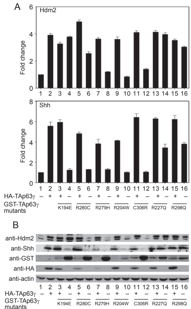
Figure 4 Effect of TAp63 \gamma mutants on TAp63 \gamma -mediated induction of Hdm2 and Shh expression. H1299 cells were transfected with wildtype TAp63 \gamma alone or co-transfected with TAp63 \gamma mutants as indicated. (A) Transcript levels of Hdm2 (upper panel) and Shh (lower panel) were detected using TaqMan-based real-time PCR. The Y-axis represents fold change in transcript levels relative to vector-transfected cells. (B) Immunoblot analysis was performed to detect the endogenous protein expression of Hdm2 and Shh and to confirm the overexpression of HA-tagged TAp63 \gamma and GST-tagged TAp63 \gamma mutants. Immunoblotting for \beta -actin served as the loading control.
