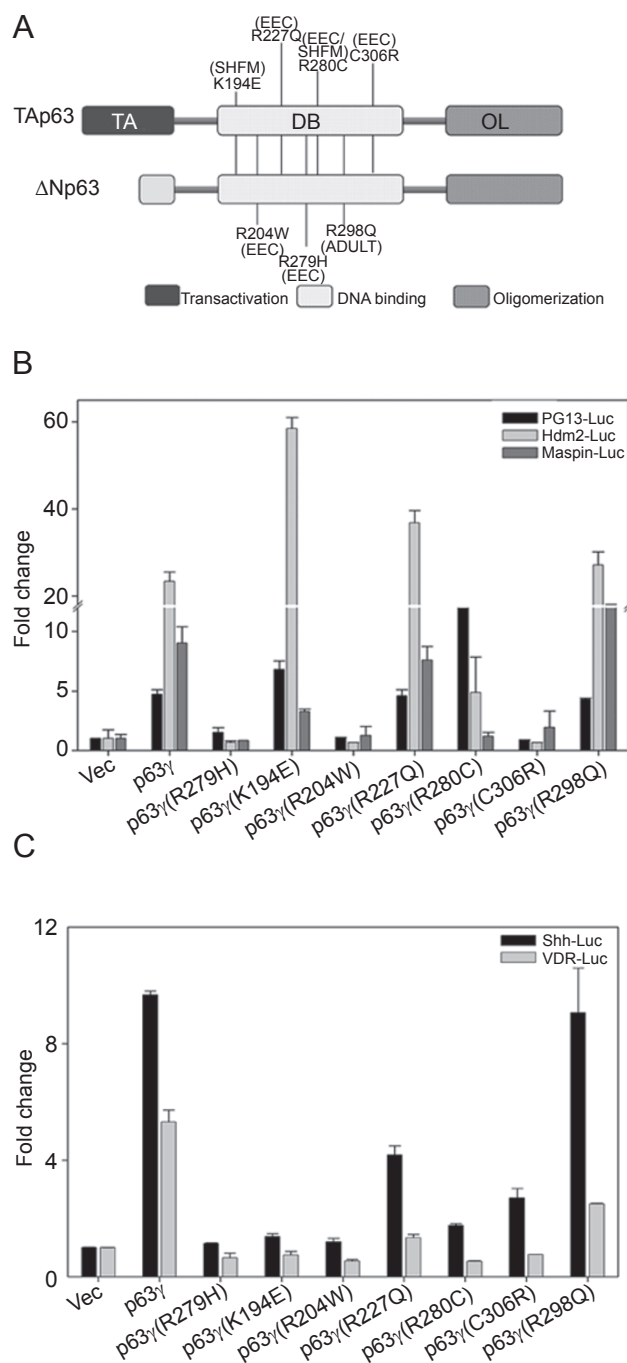
Figure 1 Differential transactivation potential of p63 mutants on p53/p63 and p63 specific reporters. (A) A schematic representation of p63 gene architecture and location of p63 missense mutations tested and the syndrome associated with each of the mutations in this study. (B and C) H1299 cells were transfected with (B) PG13-Luc, Maspin-Luc and Hdm2-Luc reporters or (C) Shh-Luc and VDR-Luc reporters alone or along with wildtype TAp63γ or TAp63γ mutants and CMV-R-Luc plasmids using lipofectamine 2000 as indicated. The ratio of firefly luciferase units to Renilla luciferase units was calculated for normalizing luciferase units to transfection efficiency. The Y-axis represents the fold change in relative luciferase units compared with empty vector.
