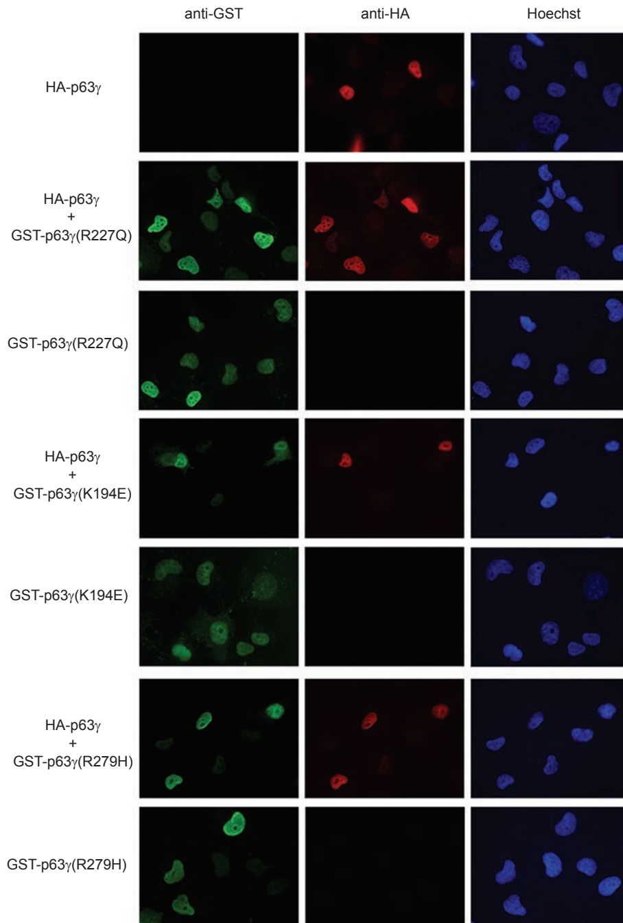
Figure 5 TAp63 \gamma mutants do not affect the localization of wildtype TAp63 \gamma . H1299 cells were transfected with HA-tagged TAp63 \gamma alone or along with GST-tagged TAp63 \gamma mutants as indicated. At 24 h post-transfection immunofluorescence assay was performed. Wildtype TAp63 \gamma and TAp63 \gamma mutant expression was detected using mouse anti-HA and rabbit anti-GST primary antibodies, respectively, and subsequently with the corresponding secondary antibodies. The nucleus was stained with Hoechst dye and the cells were examined using a fluorescence microscope.
