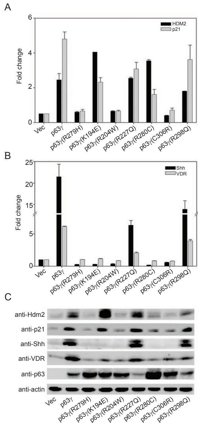
Figure 2 Differential activation of p53/p63 and p63 specific target genes by p63 mutants. (A) H1299 cells were transfected with TAp63 \gamma , TAp63 \gamma mutants or empty vector alone as indicated. At 24 h post-transfection, total RNA was extracted and (A) Hdm2 and p21; (B) Shh and VDR transcript levels were detected using TaqMan-based real-time PCR. The Y-axis represents the fold change in transcript levels relative to vector-transfected cells. (C) Immunoblot analysis was performed to confirm the overexpression of p63 and endogenous expression of Hdm2, p21, Shh and VDR using gene specific antibodies. Immunoblotting for \beta -actin served as the loading control.
