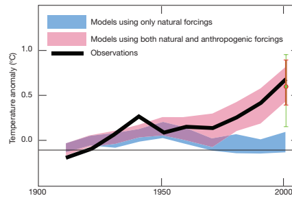
Figure 2 Comparison of observed changes in global mean surface temperature with results simulated by climate models using natural and anthropogenic forcings. Decadal averages of observations are shown for the period 1906–2005 (black) plotted against the centre of the decade and relative to the corresponding average for 1901–1950. The blue band shows the 5–95% range for 19 simulations from five climate models using only the natural forcings due to solar activity and volcanoes. The rose-coloured band shows the 5–95% range for 58 simulations from 14 climate models using both natural and anthropogenic forcings 1 . Added to the figure are I-beams denoting uncertainties. The range of the modelled increase in global mean surface temperature over the twentieth century (red) — ~0.5 to 1.0 °C, or a factor of 2 — is smaller than that of the IPCC estimate for the global mean forcing (green), given in Fig. 1, which is a factor of 4.
