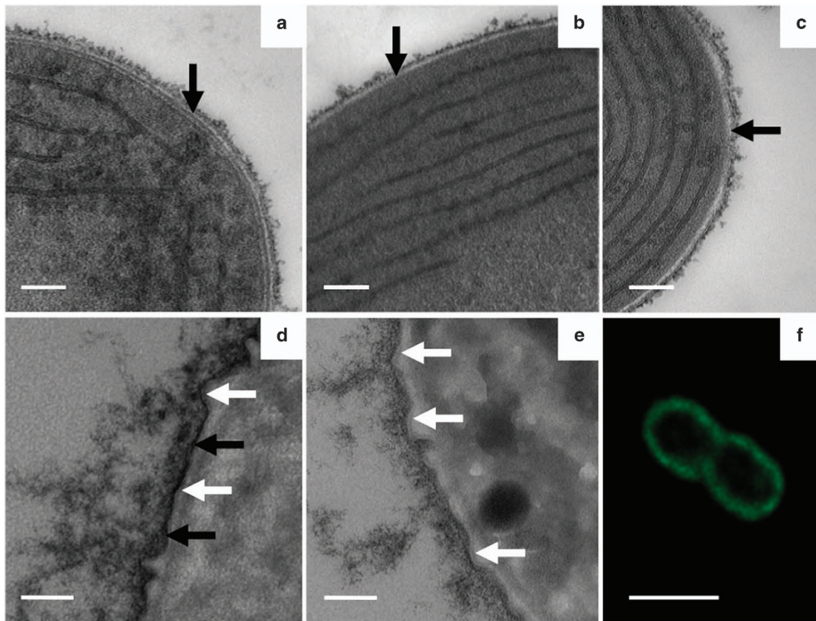
Figure 2 Transmission electron microscopy (TEM) study of cell walls in thin sections of Synechococcus 7002. (a) Wild type (WT). (b) cesA mutant. (c) WT cells incubated in a cellulase solution (200 \mu\text{g}/\text{ml} in the presence of 2 mM EDTA) for 30 min at 37 ^{\circ}\text{C} . The arrow in a indicates the electron-dense layer, and the arrows in b and c indicate its absence. Note that there is more cell-surface-associated glycocalyx material in a than in b or c. (d, e) TEM images of thin sections of Synechococcus 7002 cells stained with ruthenium red showing the changes in the cell wall and glycocalyx of WT (d) and a cesA deletion mutant (e), respectively. The black arrows indicate the possibly laminated, CesaA-dependent cellulose layer, and the white arrows indicate the thin peptidoglycan layer. Although it was easier to see on lower-magnification images (data not shown), these images show less ruthenium red staining for the cesA mutant (e), more staining for the WT (d), and much more staining for a strain overproducing CesaA (see Figure 4c). These data show that the cesA mutant had the least surface-associated polysaccharides and that the strain overproducing CesaA had the most. An electron-opaque, laminated layer near the outer membrane in WT (black arrows in d) was missing in the cesA mutant (e). This layer apparently corresponds to the cellulose layer observed between the peptidoglycan (white arrows in d and e) and outer membrane layers in thin sections in a. (f) Confocal fluorescence microscopy showing spectrally deconvoluted, Z-stack image of Synechococcus 7002 cells expressing CesaA-YFP. This image shows the absence of YFP fluorescence in the cytoplasm and thylakoid membranes, which could easily be visualized by fluorescence from chlorophyll a (data not shown). Scale bars, 100 nm (a-e) and 2 \mu\text{m} (f).
