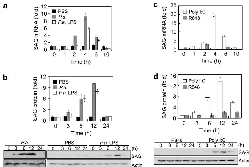
Figure 1 SAG expression is increased in J774 cells at the early stage of challenge with bacterial/viral PAMPs. (a and b) Cells were treated with heat-inactivated P. aeruginosa ( P.a. , PAO-Igiewski, 1 \times 10^6 CFU/ml), P. aeruginosa LPS ( P.a. LPS, 10 ng/ml) or phosphate-buffered saline (PBS). (c and d) Cells were treated with viral mimics; polyinosinic-polycytidylic acid (poly I:C) (10 \mu g/ml) and R848 (25 ng/ml), representing double-stranded RNA (dsRNA) and single-stranded RNA (ssRNA), respectively. (a and c) mRNA and (b and d) protein levels of SAG were induced upon treatment by P.a. LPS and poly I:C, but not by R848. Data are presented as means \pm S.D. ( n = 3 )
