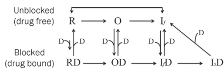
Figure 6. The model of methyl eugenol action on peripheral Na + channels. Drugs (D) can bind to Na + channels in the resting (R), open (O) and fast-inactivated ( I_i ) states. The drug-bound fast-inactivated state can switch into a drug-bound slow-inactivated state ( I_s ) under certain conditions.
