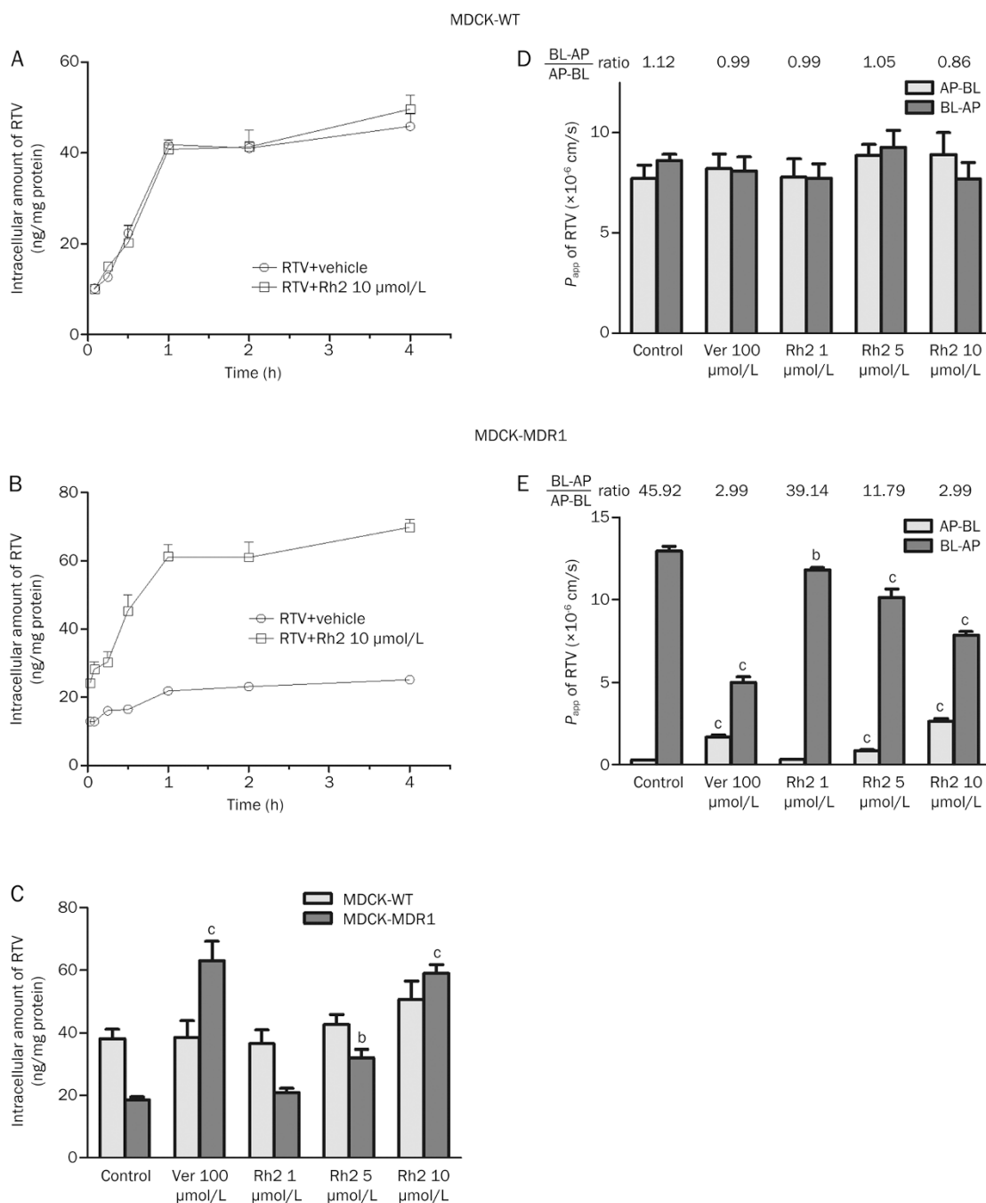
Figure 2. Effects of Rh2 on the accumulation and transport of ritonavir (RTV) in MDCK-WT and MDCK-MDR1 cells. (A) Intracellular accumulation of RTV in MDCK-WT cells treated with or without Rh2 (10 \mu\text{mol/L} ) for 5, 15, 30, 60, 120, or 240 min. (B) Intracellular accumulation of RTV in MDCK-MDR1 cells treated with or without Rh2 (10 \mu\text{mol/L} ) for 5, 15, 30, 60, 120, or 240 min. (C) The accumulation of RTV in MDCK-WT and MDCK-MDR1 cells in the presence of Rh2 or verapamil (Ver) for 60 min. (D) The transportation of RTV across MDCK-WT monolayer cells. (E) The transportation of RTV across MDCK-MDR1 monolayer cells. The cells were preincubated with Rh2 (1, 5, and 10 \mu\text{mol/L} ), or Ver (100 \mu\text{mol/L} ) for 30 min, respectively, followed by a further incubation in the presence of 2 \mu\text{mol/L} RTV for 60 min. The bars represent the mean \pm SEM of three independent experiments. b P < 0.05 , c P < 0.01 vs control. AP, apical; BL, basolateral; P_{\text{app}} , apparent permeability.
