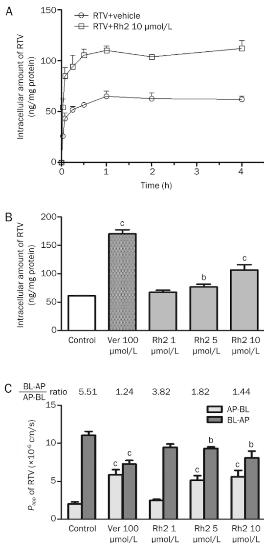
Figure 1. Effects of Rh2 on the accumulation and transport of ritonavir (RTV) in Caco-2 cells. (A) Intracellular accumulation of RTV in Caco-2 cells treated with or without Rh2 (10 µmol/L) for 5, 15, 30, 60, 120, or 240 min. (B) Intracellular accumulation of RTV in Caco-2 cells treated with verapamil (Ver) or Rh2. (C) The transportation of RTV across Caco-2 monolayers cells. The cells were preincubated with Rh2 (1, 5, and 10 µmol/L) or Ver (100 µmol/L) for 30 min, respectively, followed by a further incubation in the presence of 2 µmol/L RTV for 60 min. The bars represent the mean±SEM of three independent experiments. b P<0.05 , c P<0.01 vs control. AP, apical; BL, basolateral; P_{app} , apparent permeability.
