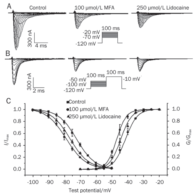
Figure 3. Effects of MFA or lidocaine on steady-state activation and inactivation of I_{Na} in Xenopus oocytes. The activation protocol was obtained from the current-voltage relationship ( 100 -ms depolarizing pulses to potentials ranging from -70 mV to -20 mV in 5 mV increments), and the inactivation curve was obtained using of a double-pulse protocol ( 100 -ms conditioning prepulses from a holding potential of -100 mV to -40 mV in 5 mV increments), followed by a test pulse to -10 mV for 100 ms. (A and B) The activation and inactivation currents of human Na_v1.5 channels expressed in Xenopus oocytes before and after superfusion of 100 \mu\text{mol/L} MFA or 250 \mu\text{mol/L} lidocaine, respectively. (C) The normalized steady-state activation and inactivation of human Na_v1.5 channels expressed in Xenopus oocytes plotted in the absence and presence of 100 \mu\text{mol/L} MFA or 250 \mu\text{mol/L} lidocaine.
