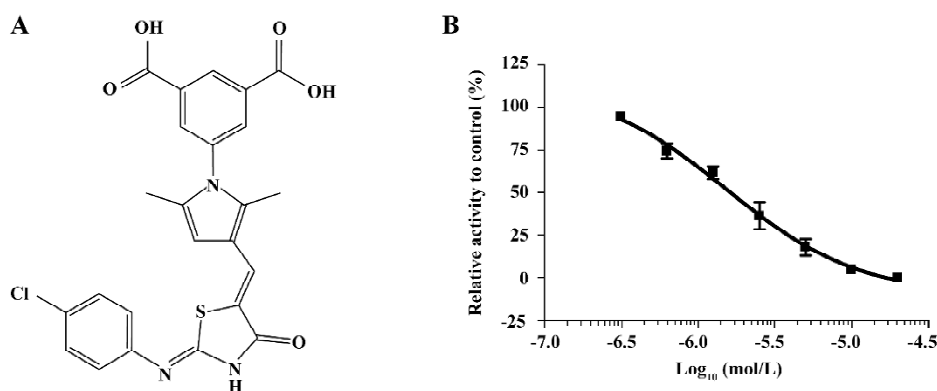
Figure 1. (A) Structure of LGH00081. (B) Dose-dependent inhibition of PTP1B by LGH00081.
