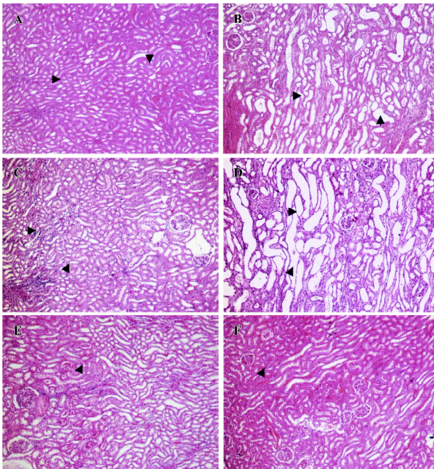
Figure 1. Light microscopy of renal tissue (5 \mu m) from Wistar Kyoto rats (A), renal failure Wistar Kyoto (B), spontaneously hypertensive rats (C), renal failure spontaneously hypertensive rats (D), control rats for experimental diabetic nephropathy (E) and experimental early diabetic nephropathy rats (F). Hematoxylin & eosin staining ( \times 200 ). In renal failure rats either spontaneously hypertensive rats or Wistar Kyoto rats, a severe destruction of tubular structure was observed. However, in diabetic nephropathy rat there was no significant tubular damage observed. The arrows are indicating the areas with either normal tubular structure or damages.
