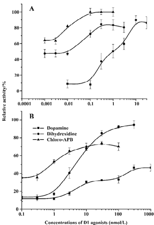
Figure 2. The activities of D1-like receptor agonists in cell lines expressing human D1 or D5 receptors. (A) D1/CRE/TA/CHO cells were incubated with D1-like receptor agonists for 6 h; (B) D5/CRE/TA/CHO cells were incubated with D1-like receptor agonists for 6 h.
