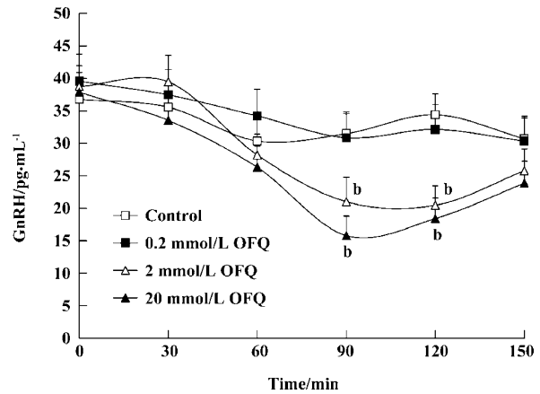
Figure 1. Dose-response curves for the effect of OFQ on GnRH release from medial basal hypothalamic slices from OVX rats. OFQ and ACSF were administered at t=0 . n=5 . Mean \pm SD. b P < 0.05 vs control.
