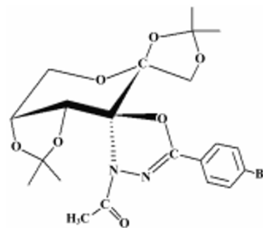
Figure 1. Chemical structure of GLB.
