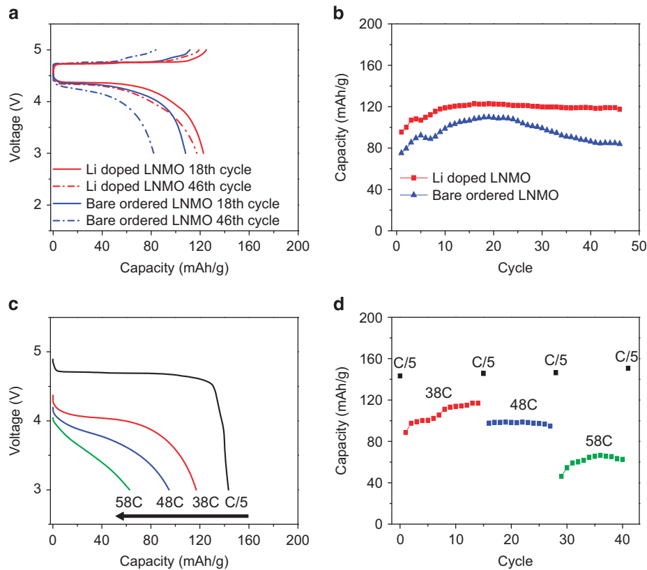
Figure 3 Electrochemical properties of the two samples. (a) The voltage curve of the bare sample and the Li-doped sample. (b) Capacity retention of both samples at discharge rate at 10C. (c) Rate capability curve of Li-doped sample without the voltage hold at the end of charge. (d) Capacity retention of Li-doped sample. Charge rate was C/5 without holding the voltage and discharge rates were different. Cutoff voltages were set from 3 to 5V.
