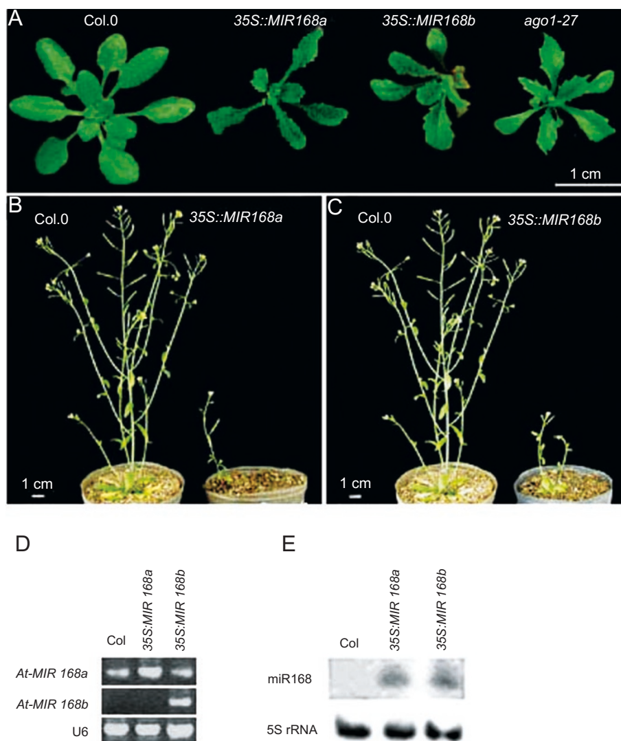
Figure 6 Development defects caused by overexpressing of At-MIR168a and At-MIR168b , and expression levels of miR168 precursors and mature miR168 in 35S::MIR168a and 35S::MIR168b transformants. (A)-(C) Similar ago1 mutant phenotypes were observed in both 35S::MIR168a and 35S::MIR168b transformants. (D) MiR168 precursors accumulation detected using RT-PCR in transgenic plants. The At-MIR168b precursor could be detected in 35S::MIR168b transformants. (E) Mature miR168 accumulation in both 35S::MIR168a and 35S::MIR168b transformants.
