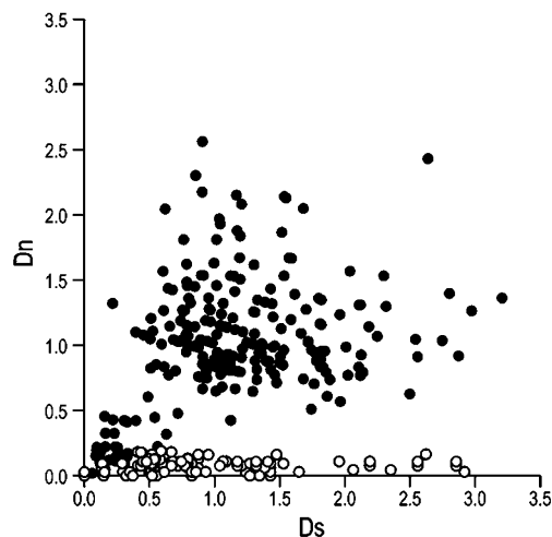
Figure 1 Pairwise comparison of nonsynonymous substitutions per nonsynonymous site ( D_n ) versus synonymous substitutions per synonymous site ( D_s ) among L. parishii S-RNases. Open symbols indicate comparisons including the conserved regions C3 and C4, whereas closed symbols are for HVa and HVb regions (Ioerger et al , 1991).
