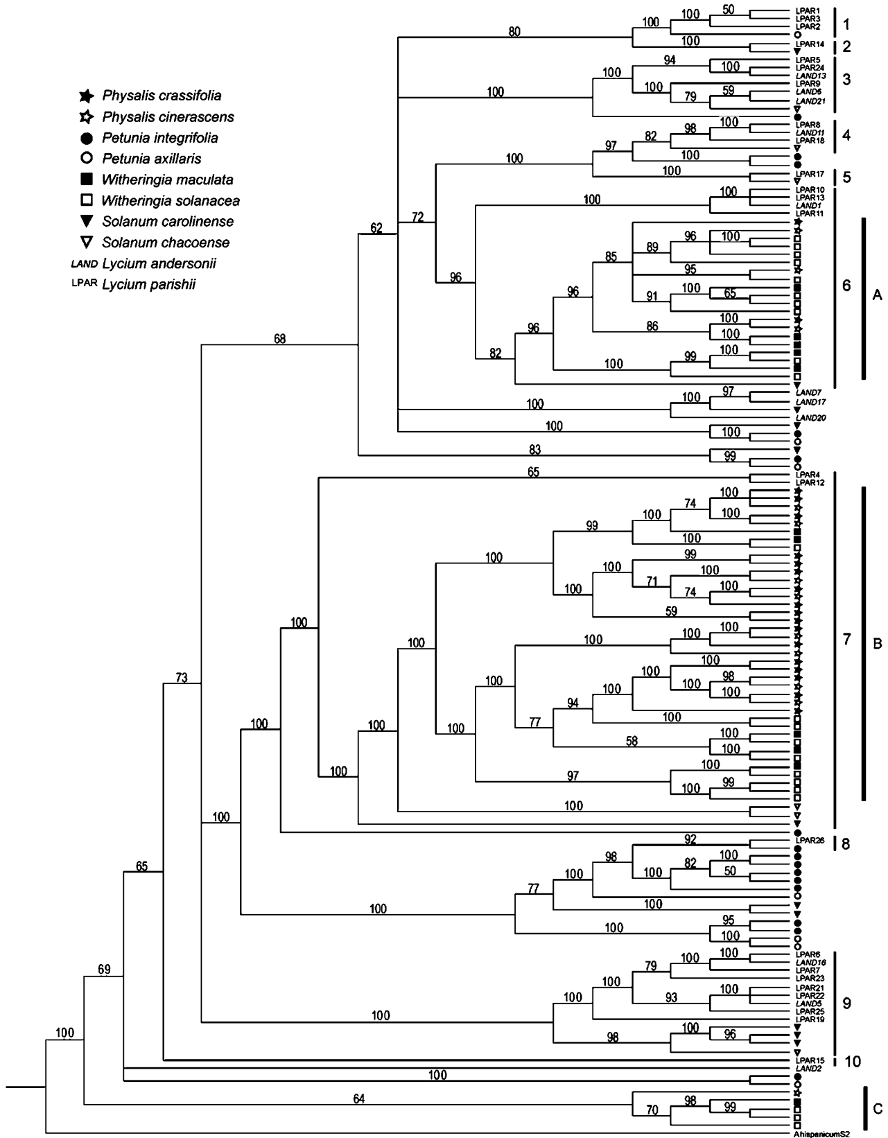
Figure 4 Bayesian genealogy including 138 S-RNase sequences from Solanaceae. Sequences for alleles from L. andersonii , Petunia spp., Physalis spp., Solanum spp., and Witheringia spp. were taken from GenBank (see Methods for accession numbers). Posterior probabilities are indicated above the branches. Clades 1–10 are L. parishii TG lineages and clades A–C are the three lineages including all Witheringia and Physalis S-RNases.
