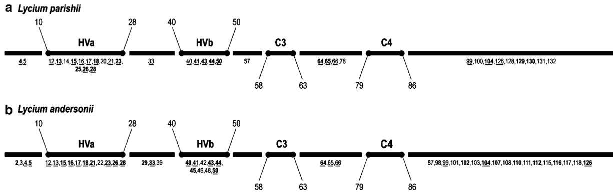
Figure 2 Schematic structure of the S-RNase gene between conserved regions C2 and C5 (Ioerger et al. , 1991) in (a) L. parishii and (b) L. andersonii . Regions are drawn to scale and the AA positions of the hypervariable (HVa and HVb) and conserved regions (C3 and C4) are indicated above or below the regions, respectively. Numbers directly below a region are those AA sites reported to be under positive selection using site-specific analyses in PAML. Those sites in bold had a probability of positive selection >90%, whereas others had probabilities between 50 and 90%. Underlined sites represent those shared between L. parishii and L. andersonii .
