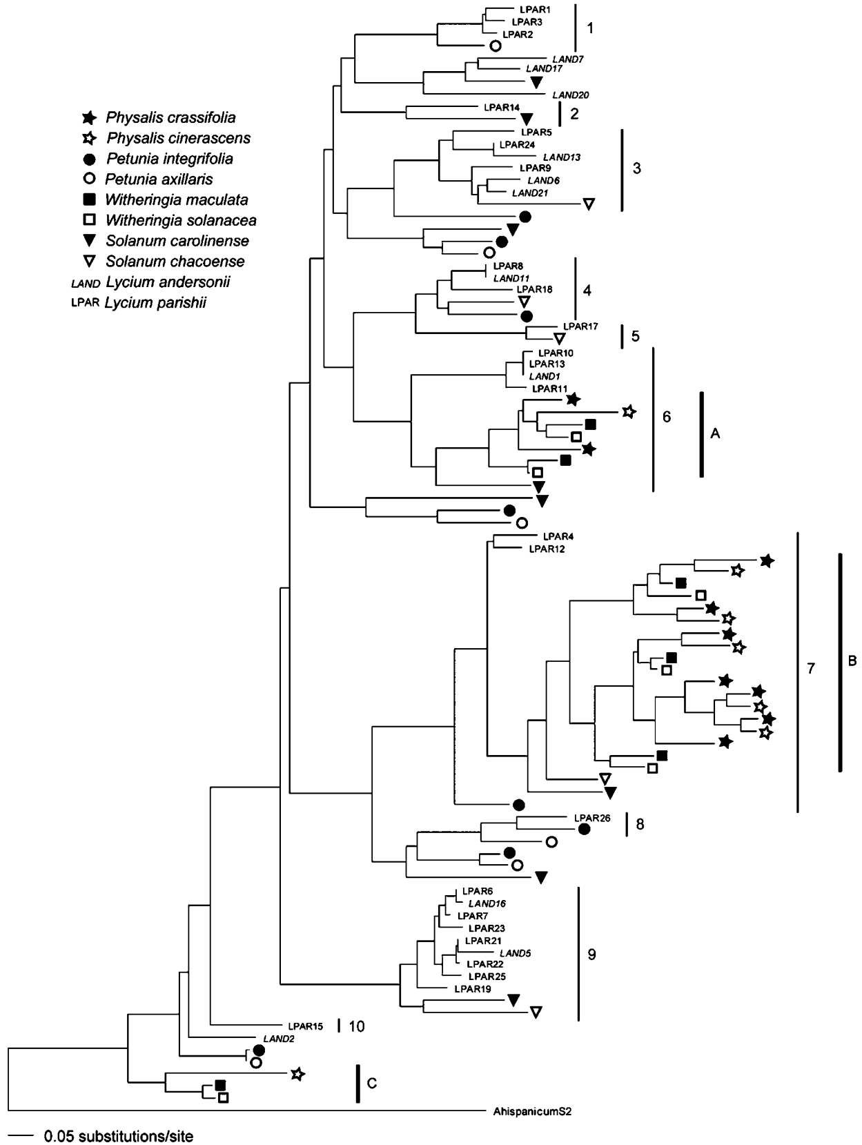
Figure 3 ML genealogy of 90 S-RNase sequences from Solanaceae. The 90 sequences were selected from a larger set of L. andersonii , Petunia spp., Physalis spp., Solanum spp., and Witheringia spp. S-RNases obtained from GenBank (see Methods for accession numbers and sampling strategy). Clades 1–10 are L. parishii TG lineages and clades A–C are the three lineages including all Witheringia and Physalis S-RNases.
